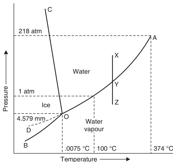
Fig. 11.1 The phase-diagram for water (not to scale).
