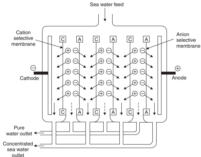
Fig. 17.7 Electrodesialysis cell.
