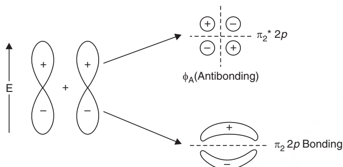
Fig. 2.24 \pi -Bonding.
