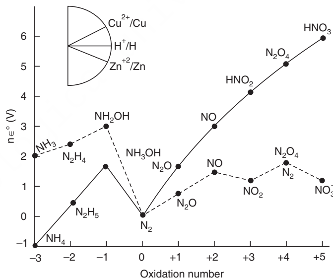
Fig. 10.3 (b) Frost diagram for nitrogen (N).
