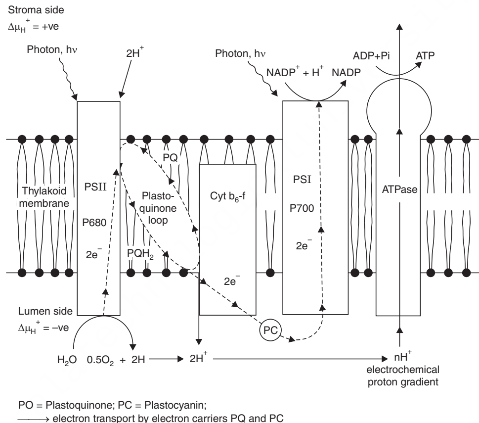
Fig. 25.8 Schematic representation of energy transduction by reaction centres PS-II and PS-I in the noncyclic photosynthetic reaction process (According to Tanz and Zieger, "Plant Physiology" Benjamin/Cummings, Redwood City, CA. (1991).
