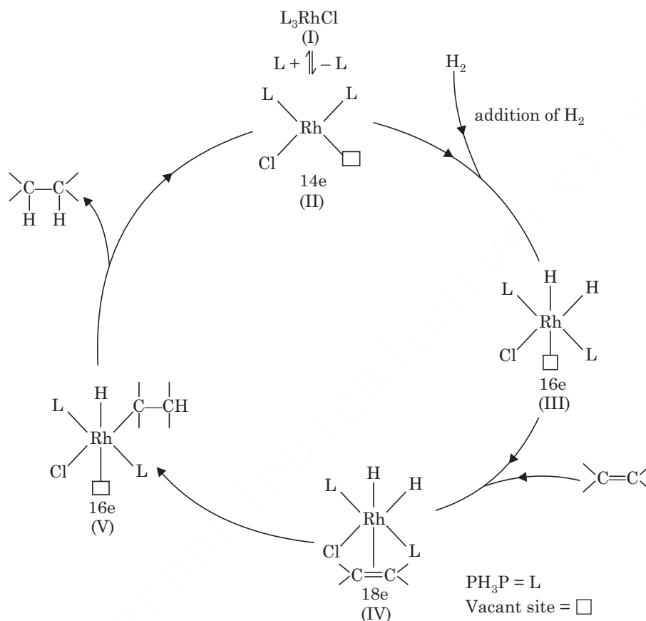
Fig. 6.7 Catalytic applications of organometallics.
