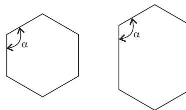
Fig. 22.1 Interfacial angle.
