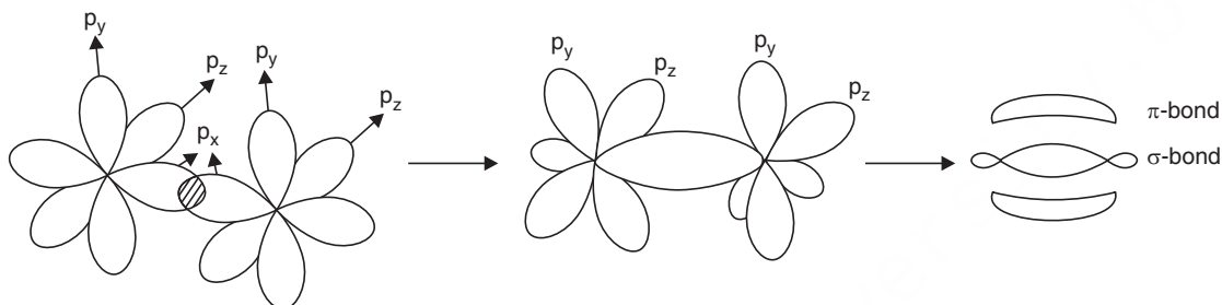
Fig. 2.7 \sigma and \pi bonds in \text{N}_2 molecule.
