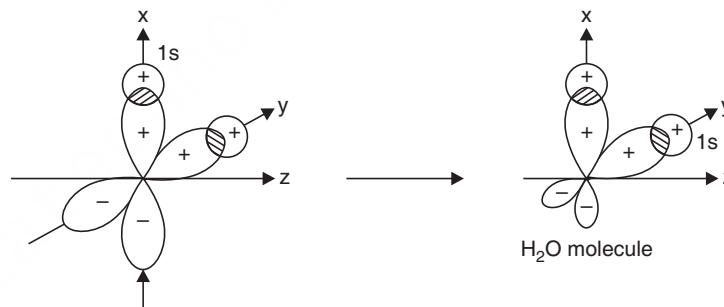
Fig. 2.5 Formation of \text{H}_2\text{O} molecule.
