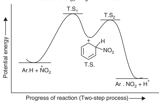
Potential energy diagram for nitration
