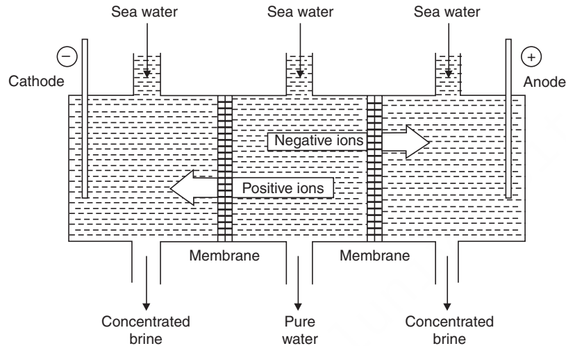
Fig. 17.6 Line diagram of electrodesialysis.
