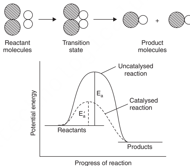
Fig. 6.1 Progress of reaction.
