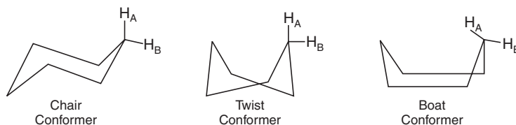
Fig. 7.4 (c) Conformers of cyclohexane.
