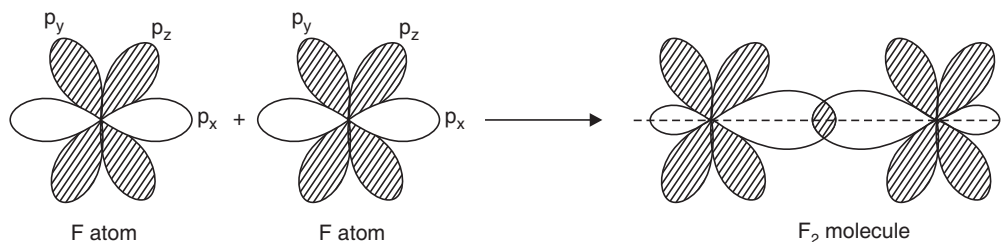
Fig. 2.6 p_x - p_x overlapping along the axis to form \text{F}_2 molecule.
