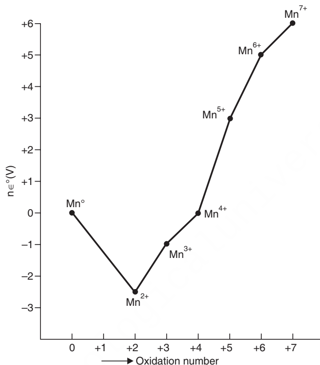
Fig. 10.20 Frost diagram for Mn in acidic pH.
