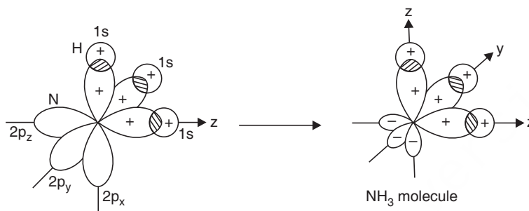
Fig. 2.4 (b) Formation of \text{NH}_3 molecule.
