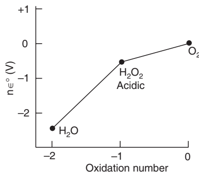
Fig. 10.4 Frost diagram for the system \text{O}_2 \rightarrow \text{O}_2^{-2} \rightarrow 2\text{O}^{-2} .
