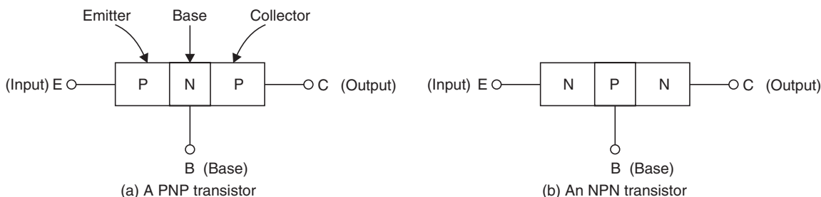
Fig. 22.16 Transistors.
