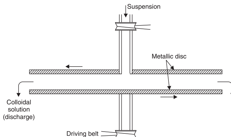
Fig. 12.2 Colloidal mill.
