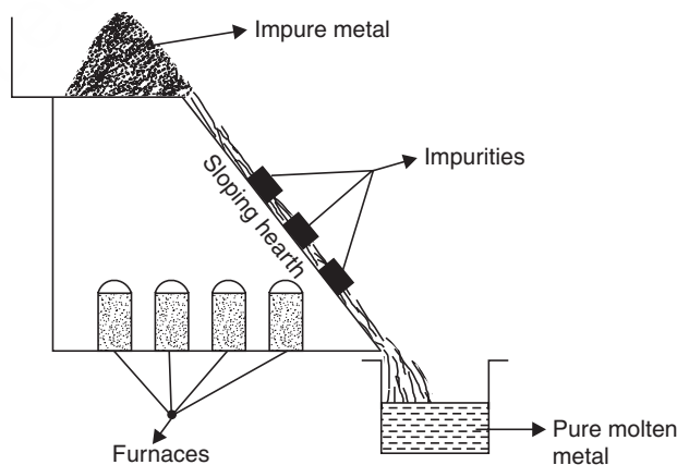
Fig. 14.11 Refining of metal by Liquation.
