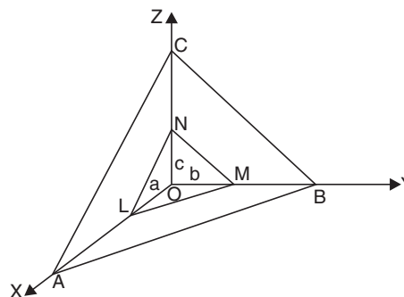
Fig. 22.2 Intercepts of crystallographic planes.
