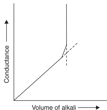
Fig. 9.10 (b) Changes in conductivity during titration of a weak acid ( \text{CH}_3\text{COOH}(\text{aq}) ) with a strong base ( \text{NaOH}(\text{aq}) ).
