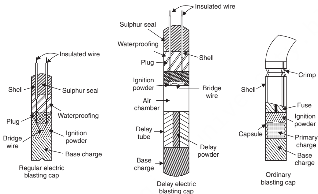
Fig. 16.1 Three types of blasting caps.
