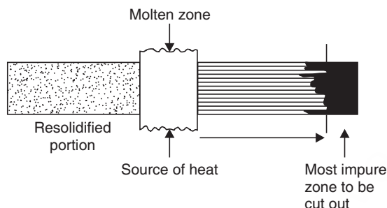
Fig. 14.12 Zone refining.
