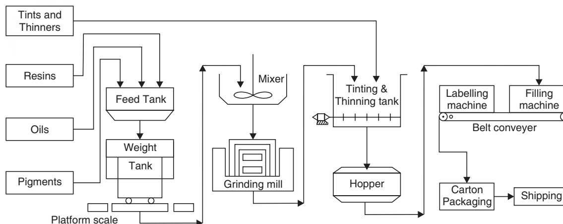
Fig. 21.1 A flow diagram of mixing of a paint.
