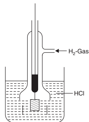
Fig. 10.6 Hydrogen Electrode.
