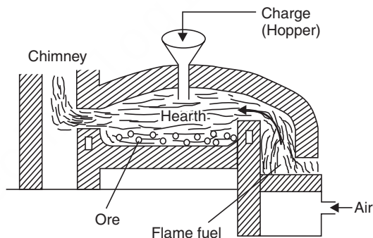
Fig. 14.6 Reverberatory furnace.
