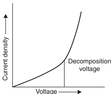
Fig. 10.13 Decomposition Potential.
