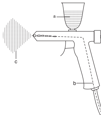
Fig. 15.1 Adhesive application by means of a spray gun (a) Adhesive (b) Compressed air (c) Atomized adhesive.
