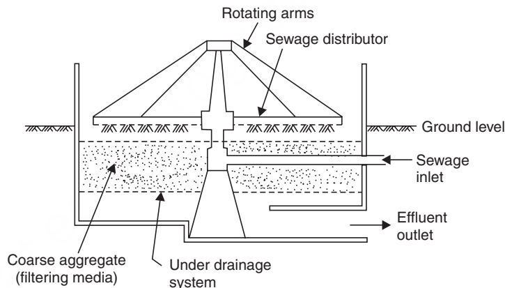
Fig. 27.4 Trickling filter.
