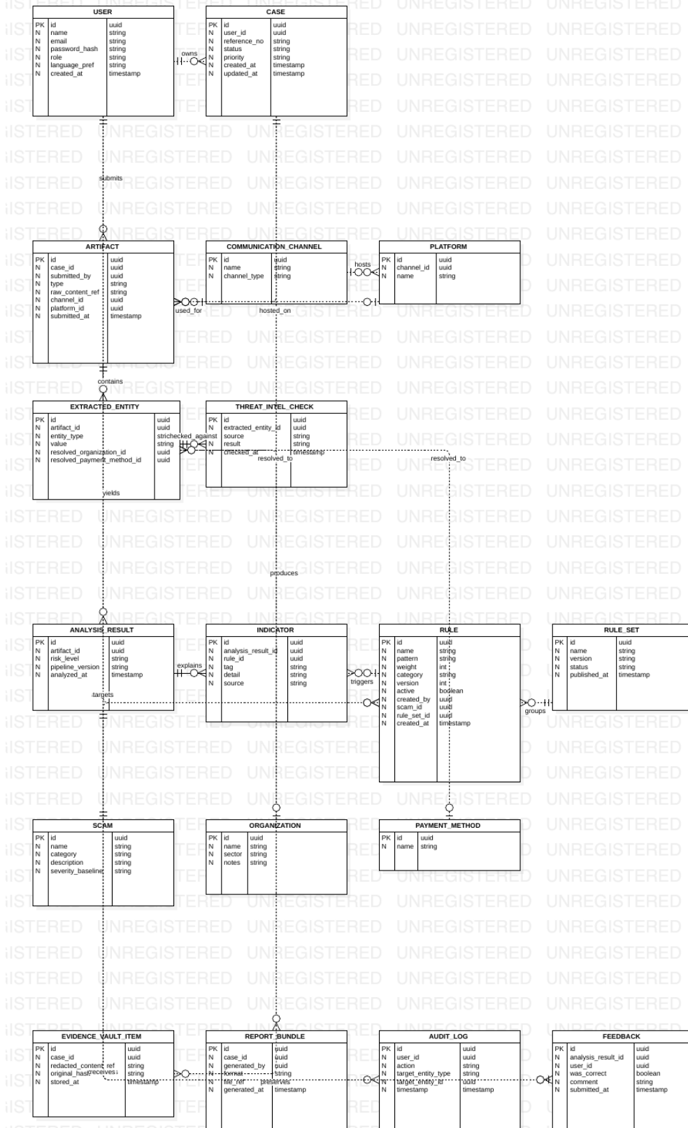
Figure B-1 — TrustLens entity relationship model
