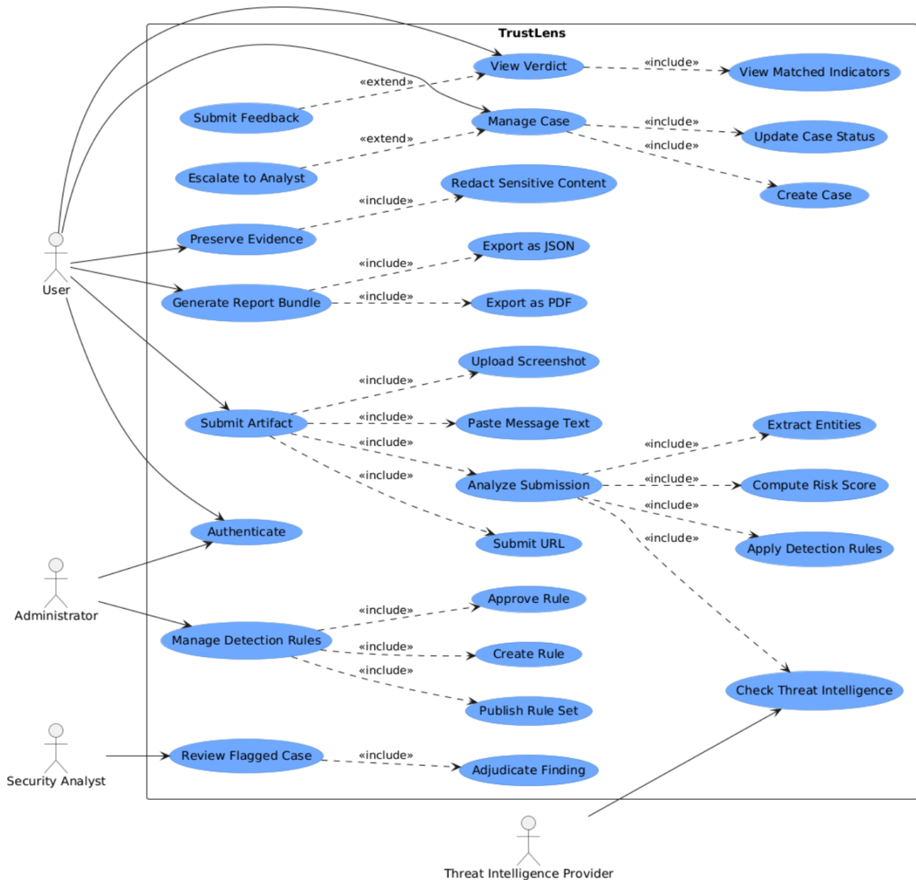
Figure B-5 — TrustLens use case diagram
