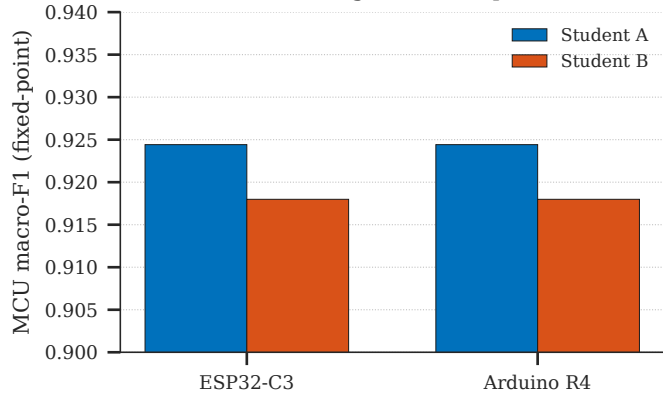
(b) MCU macro-F1 (agree=1.0 all pairs)
