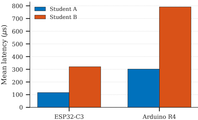
(a) Full-test HIL latency
