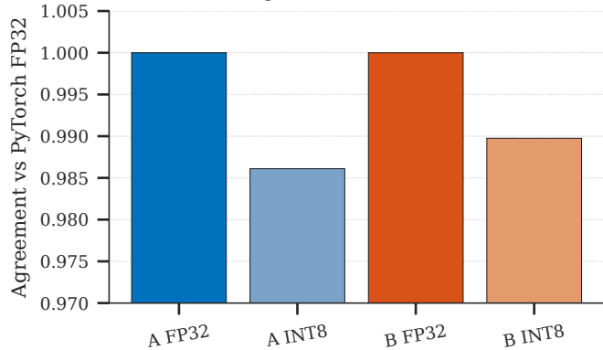
(b) Prediction agreement
