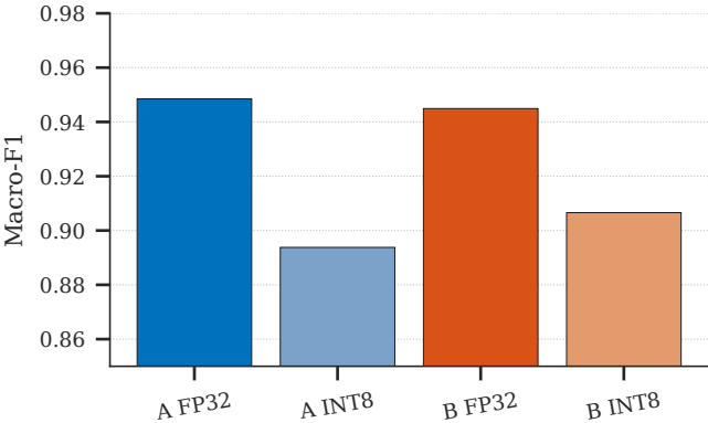
(a) Host runtime macro-F1 (U-DC)
