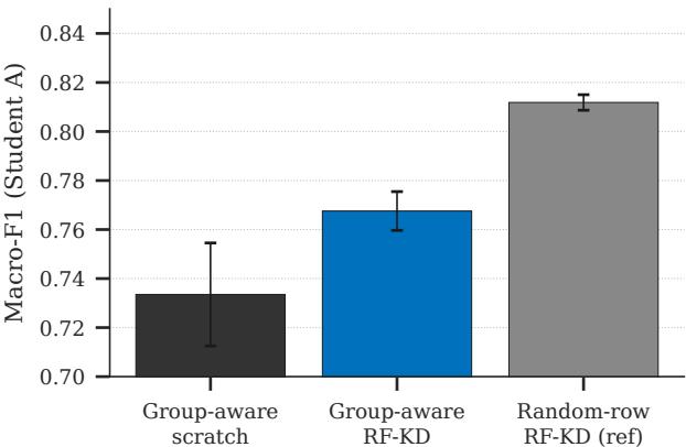
Edge-IIoTset secondary (pre-split leak audit 17.0%)
