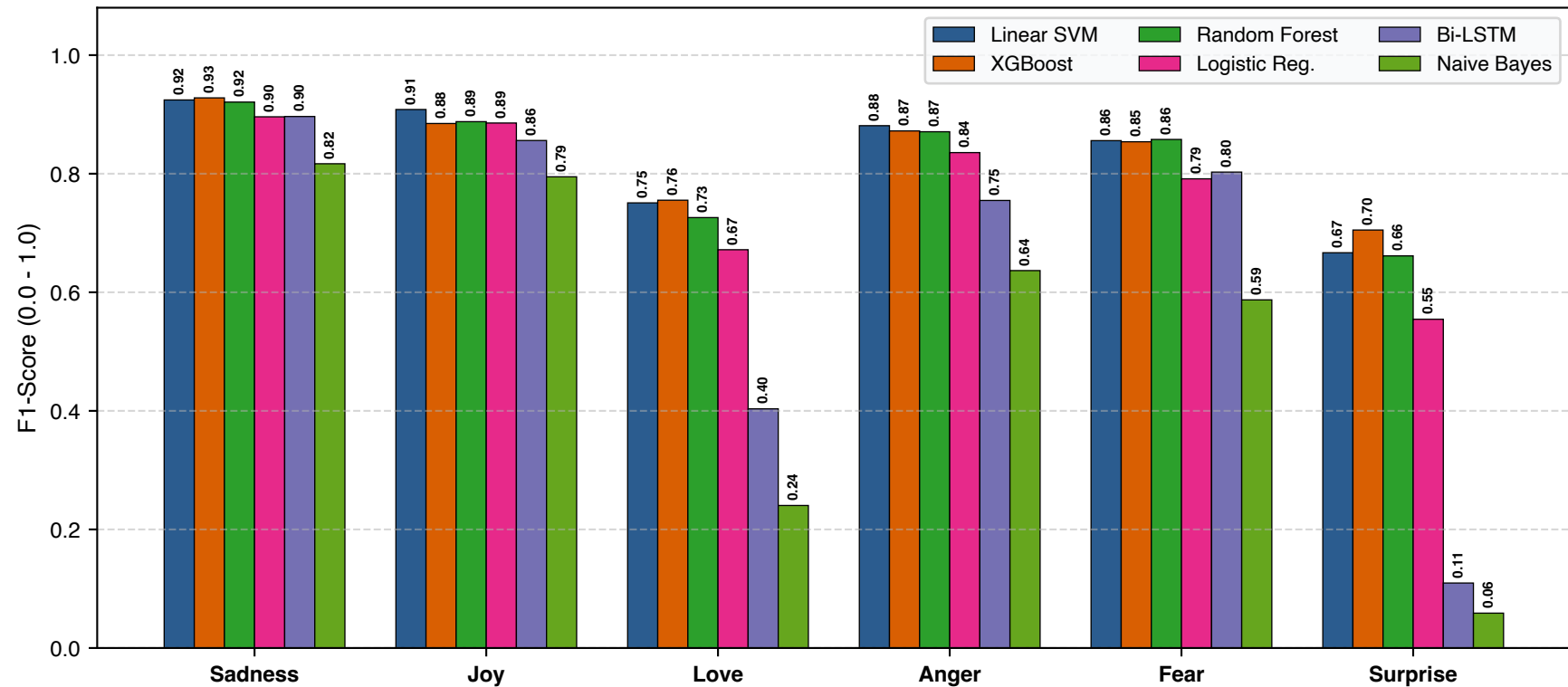
Per-Class F1-Score Breakdown Across Evaluated Models Severe Performance Degradation in Minority Emotion Classes (Love: n=159, Surprise: n=66)
