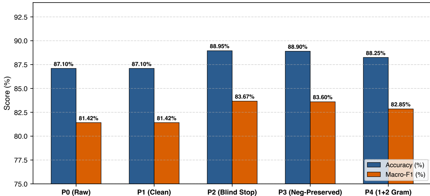
N-Gram and Preprocessing Pipeline Ablation (Random Forest 100 Trees) Accuracy and Macro-F1 across Configurations P0 through P4
