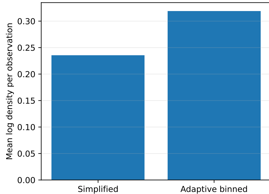
Test log-likelihood
