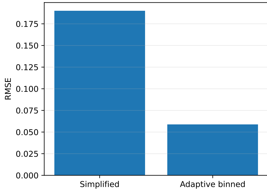
Conditional tau RMSE
