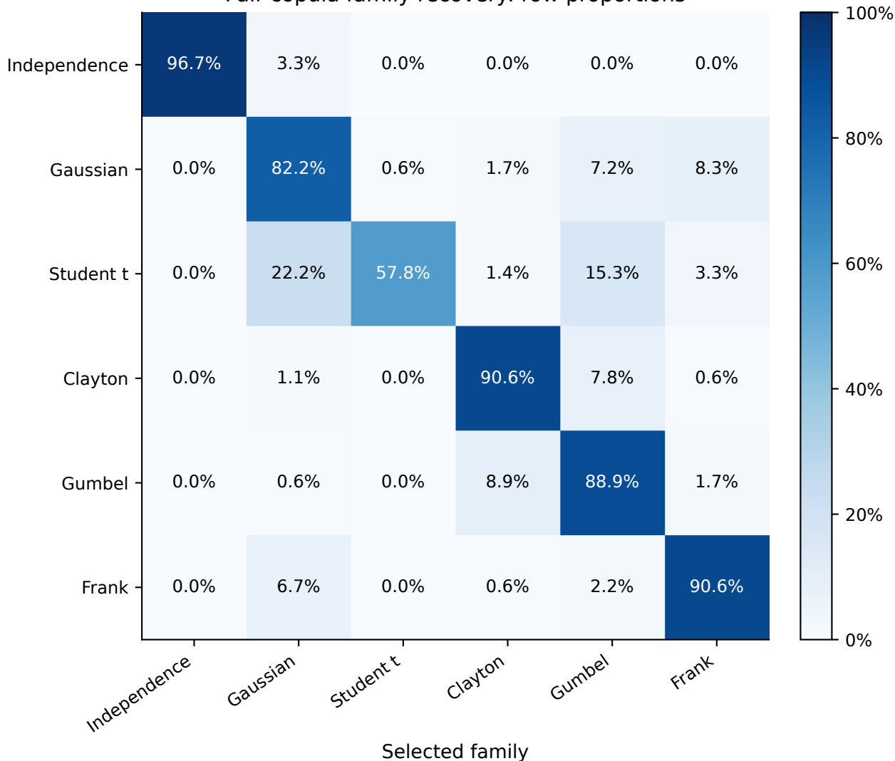
Pair-copula family recovery: row proportions
