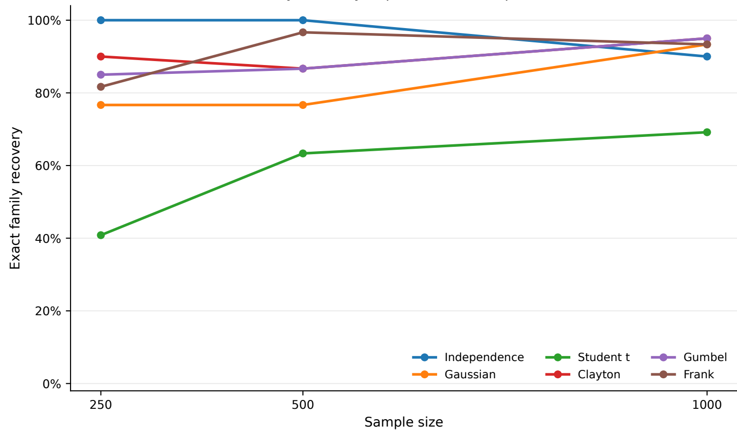
Family recovery improves with sample size
