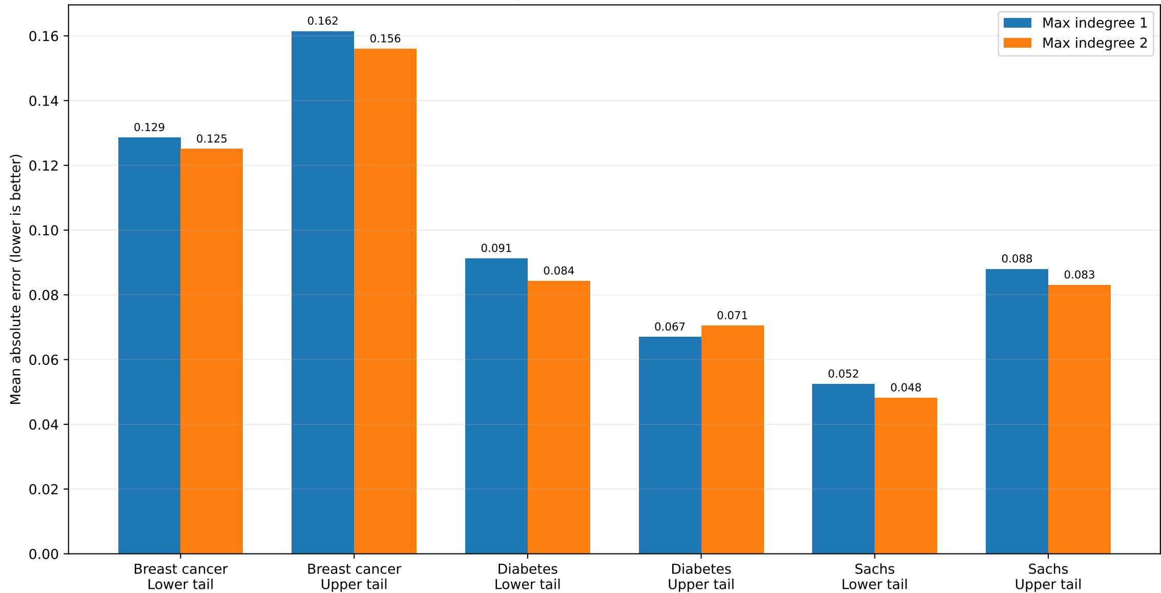
Tail-dependence reconstruction error
