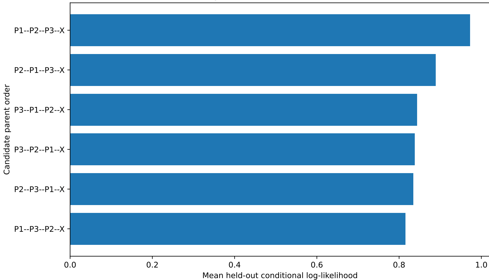
Indegree-three D-vine order selection
