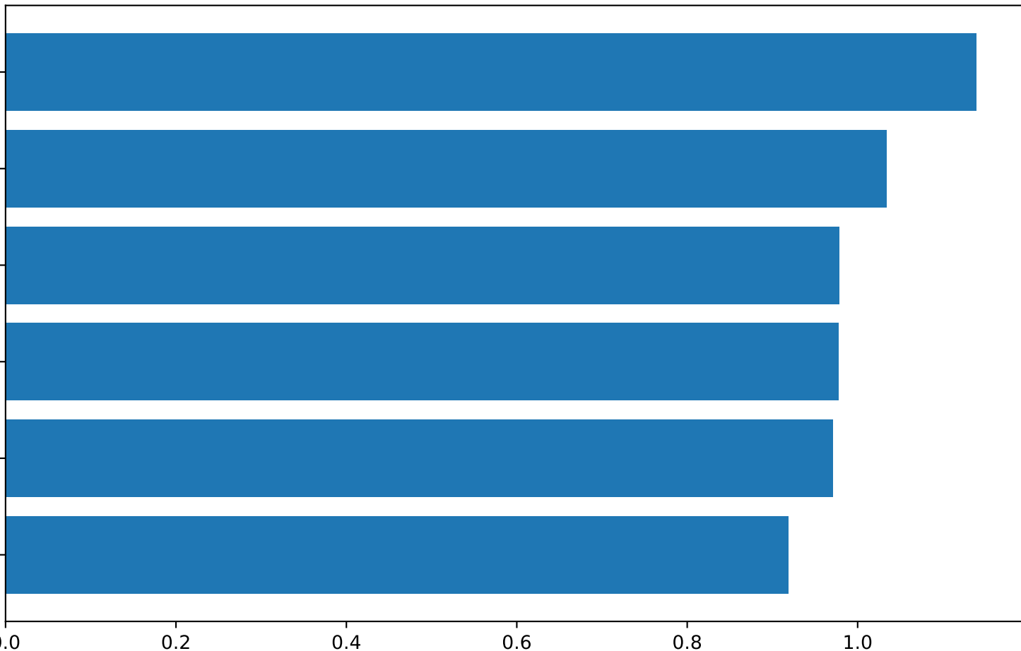
Indegree-three D-vine order selection
