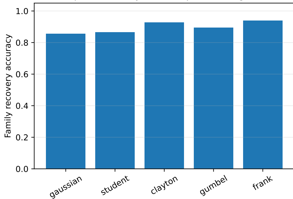
Copula recovery after empirical marginals
