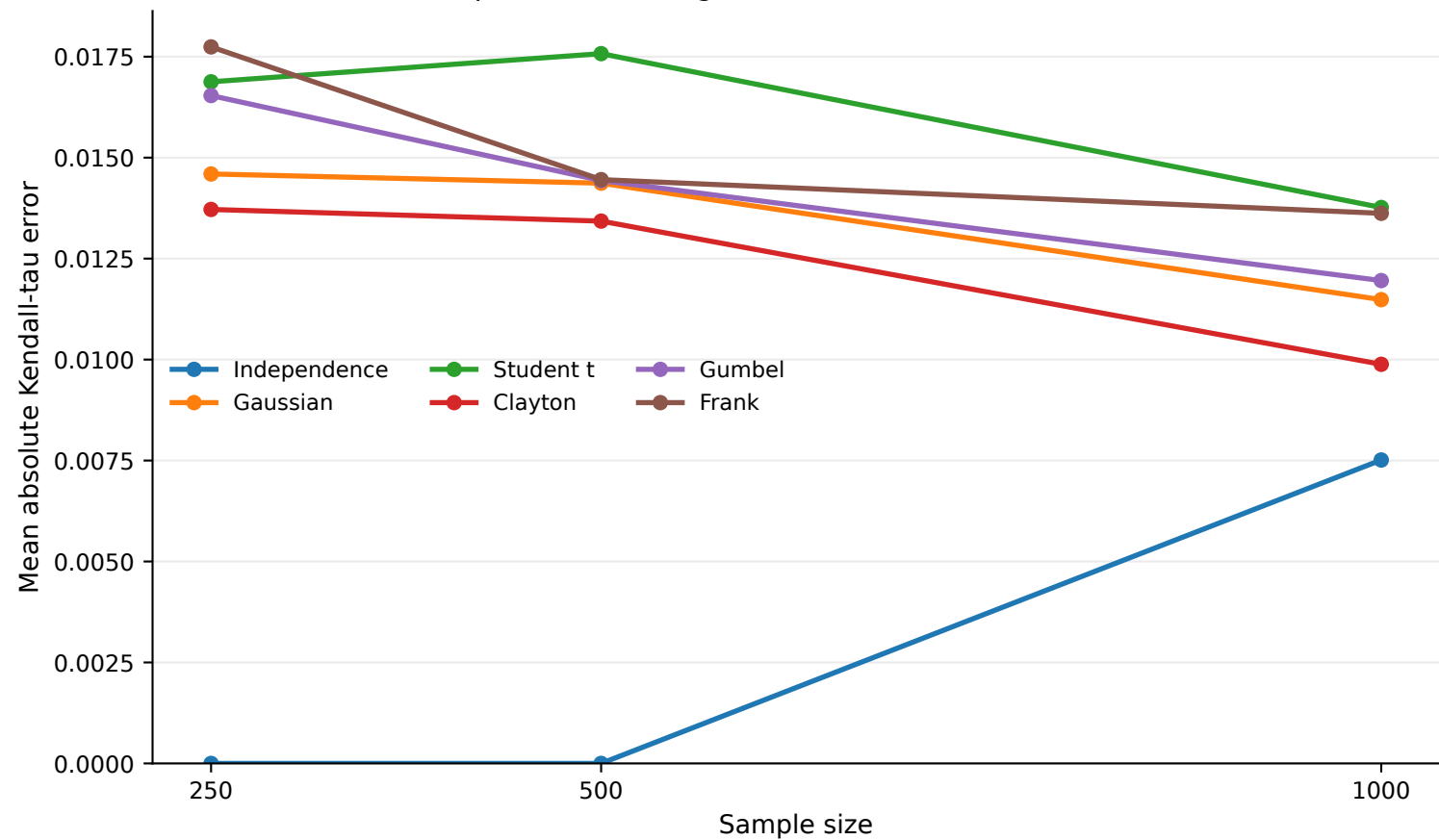
Dependence-strength estimation remains accurate
