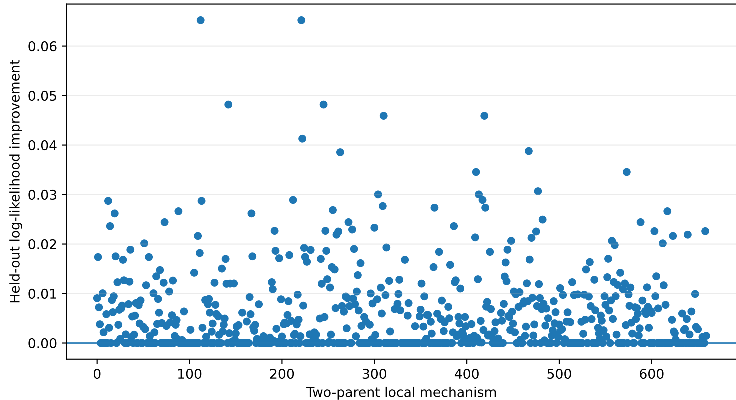
Selected conditional model versus simplifying assumption
