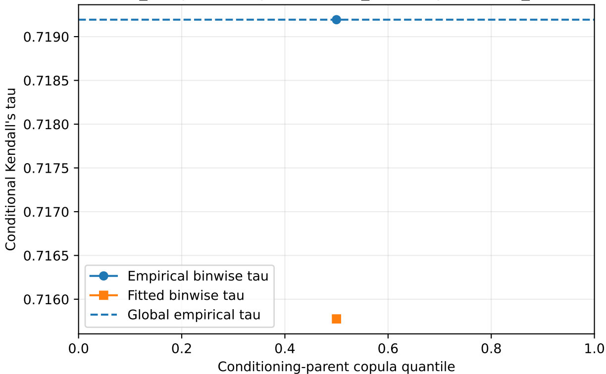
mean_compactness given ['mean_concavity', 'texture_error']
