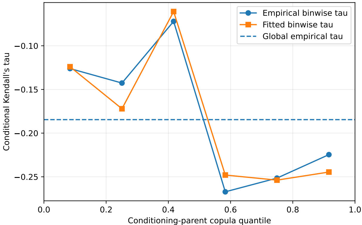
mean_compactness given ['mean_concavity', 'worst_radius']
