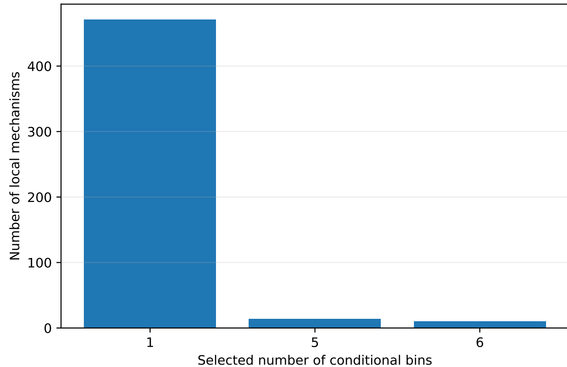
Adaptive conditional-copula model selection
