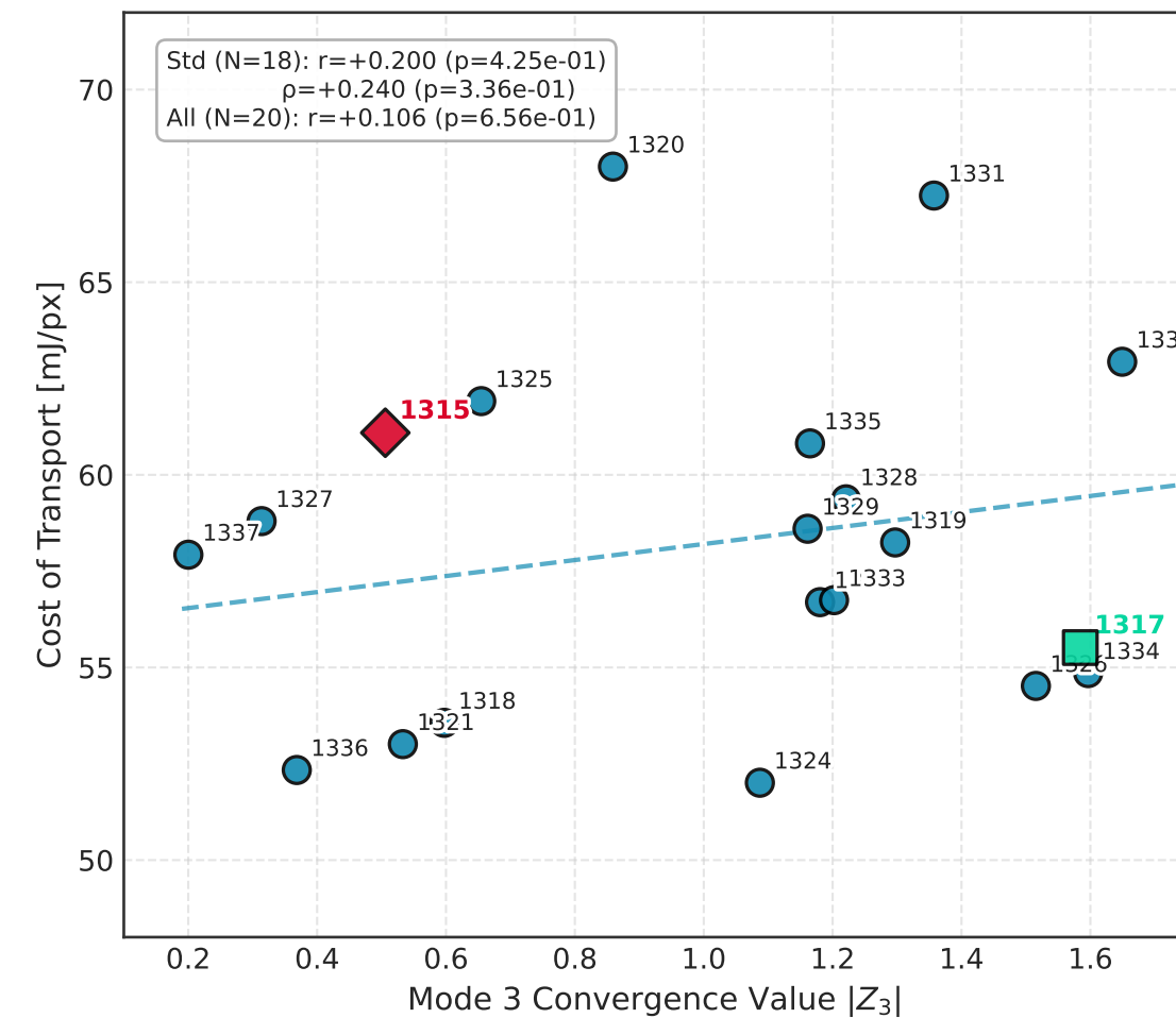
Mode 3 ( |Z_3| ) vs. Cost of Transport
