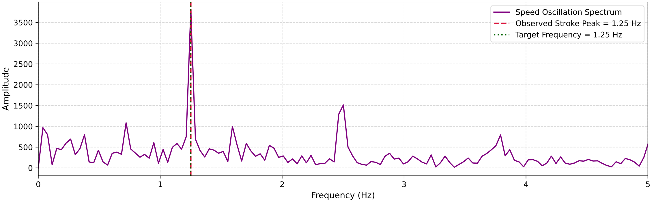
Velocity Oscillation Spectrum (FFT)
