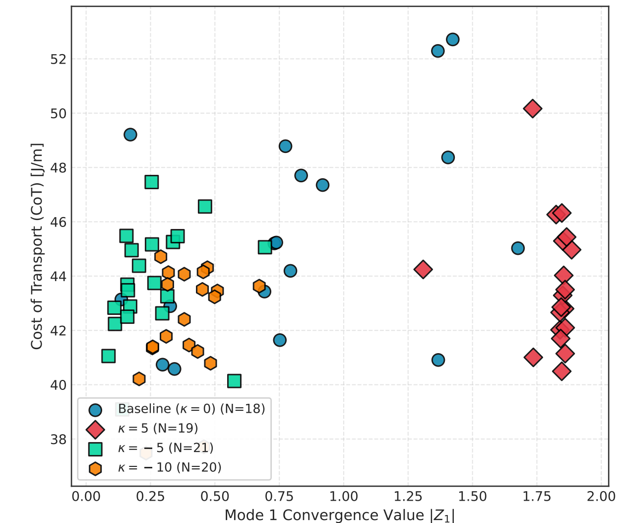
Mode 1 ( |Z_1| ) vs. Cost of Transport
