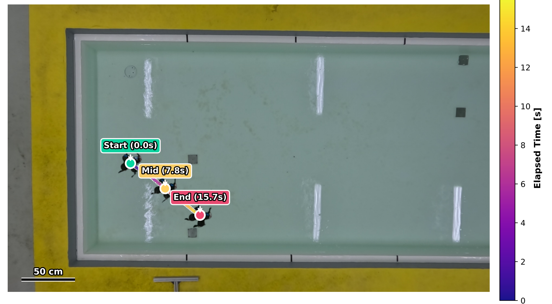
\kappa = -10 (GX011401) Speed: 5.15 cm/s, Dist: 0.82 m, CoT: 41.78 J/m
