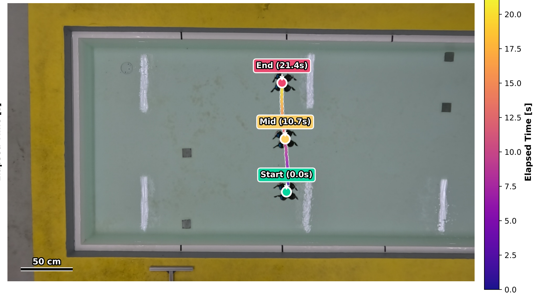
\kappa = 5 (GX011386) Speed: 4.96 cm/s, Dist: 1.09 m, CoT: 43.29 J/m
