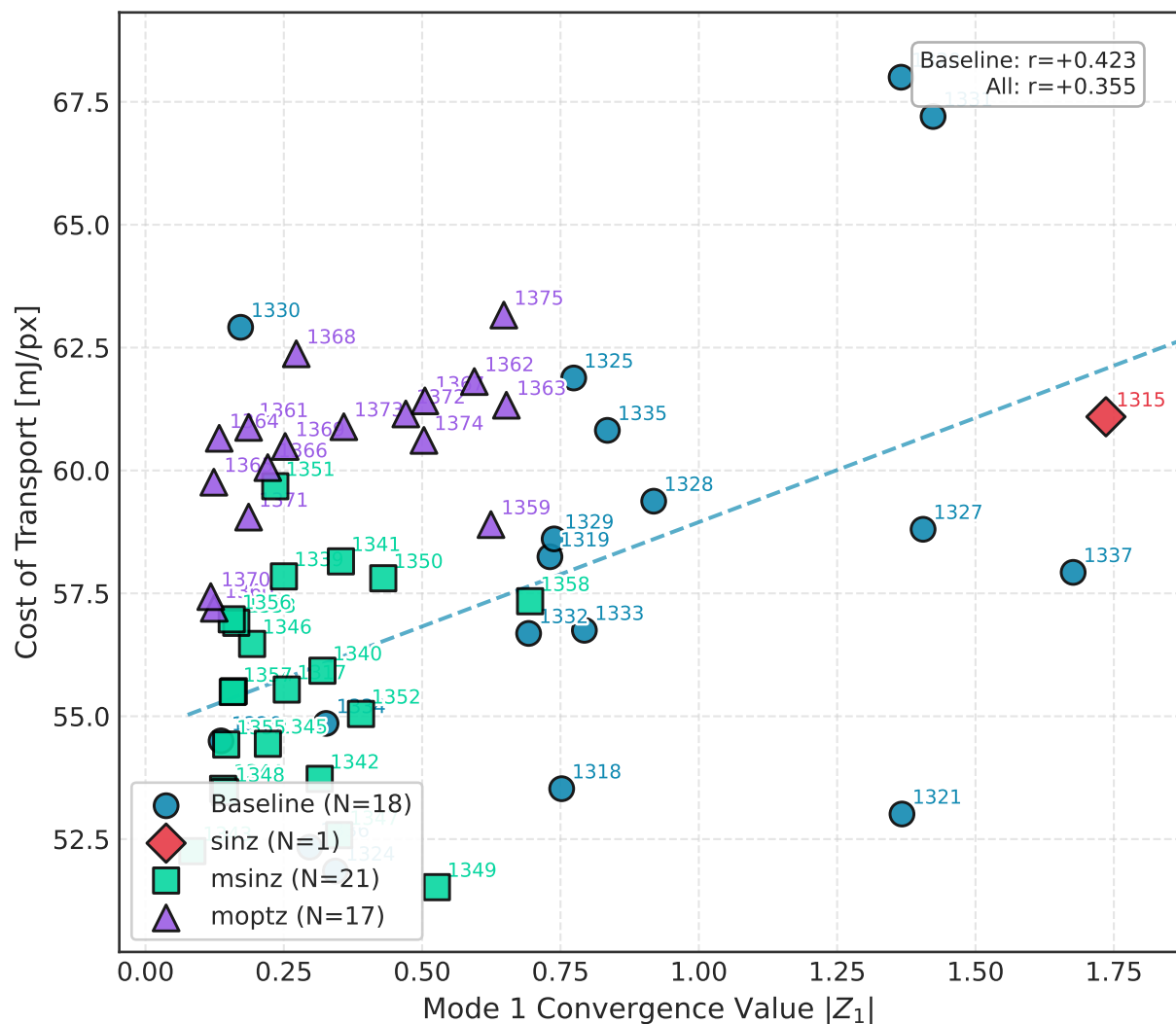
Mode 1 ( |Z_1| ) vs. Cost of Transport
