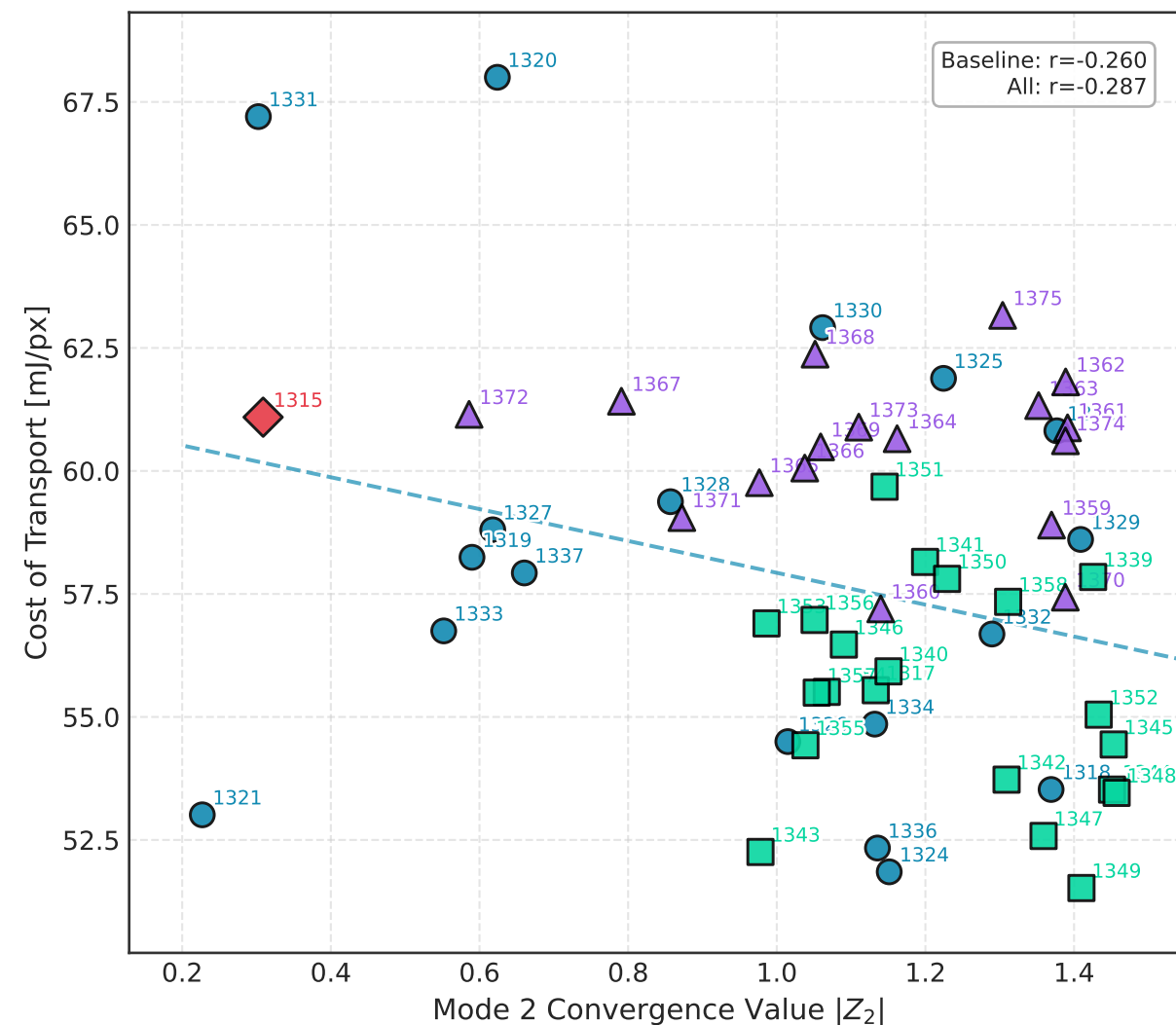
Mode 2 ( |Z_2| ) vs. Cost of Transport
