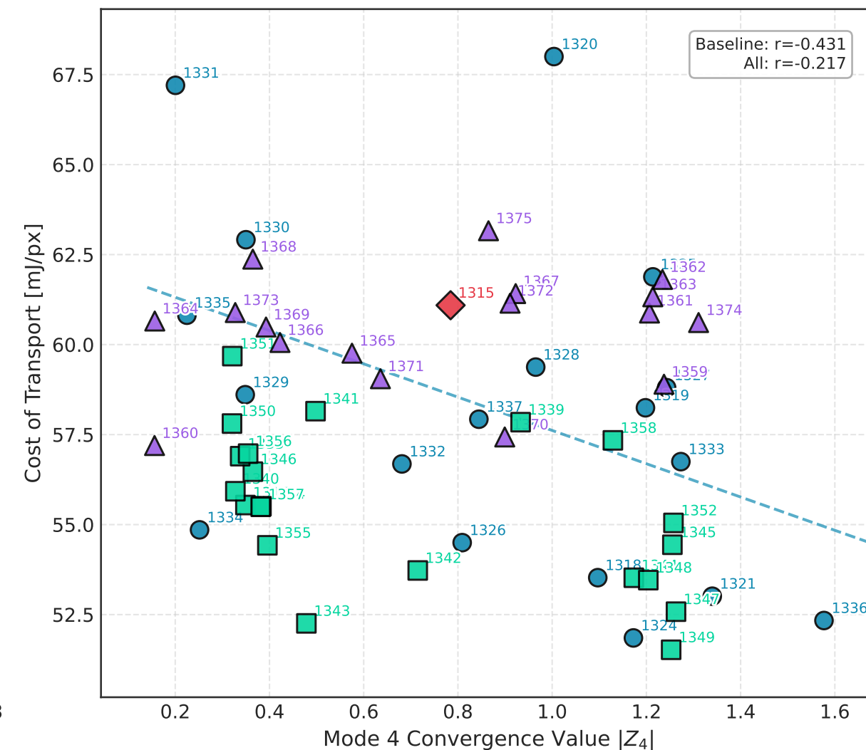
Mode 4 ( |Z_4| ) vs. Cost of Transport
