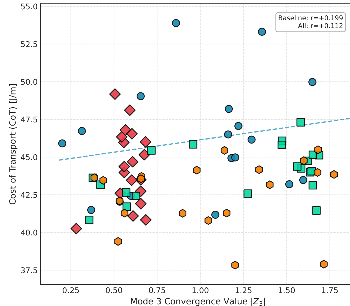
Mode 3 ( |Z_3| ) vs. Cost of Transport
