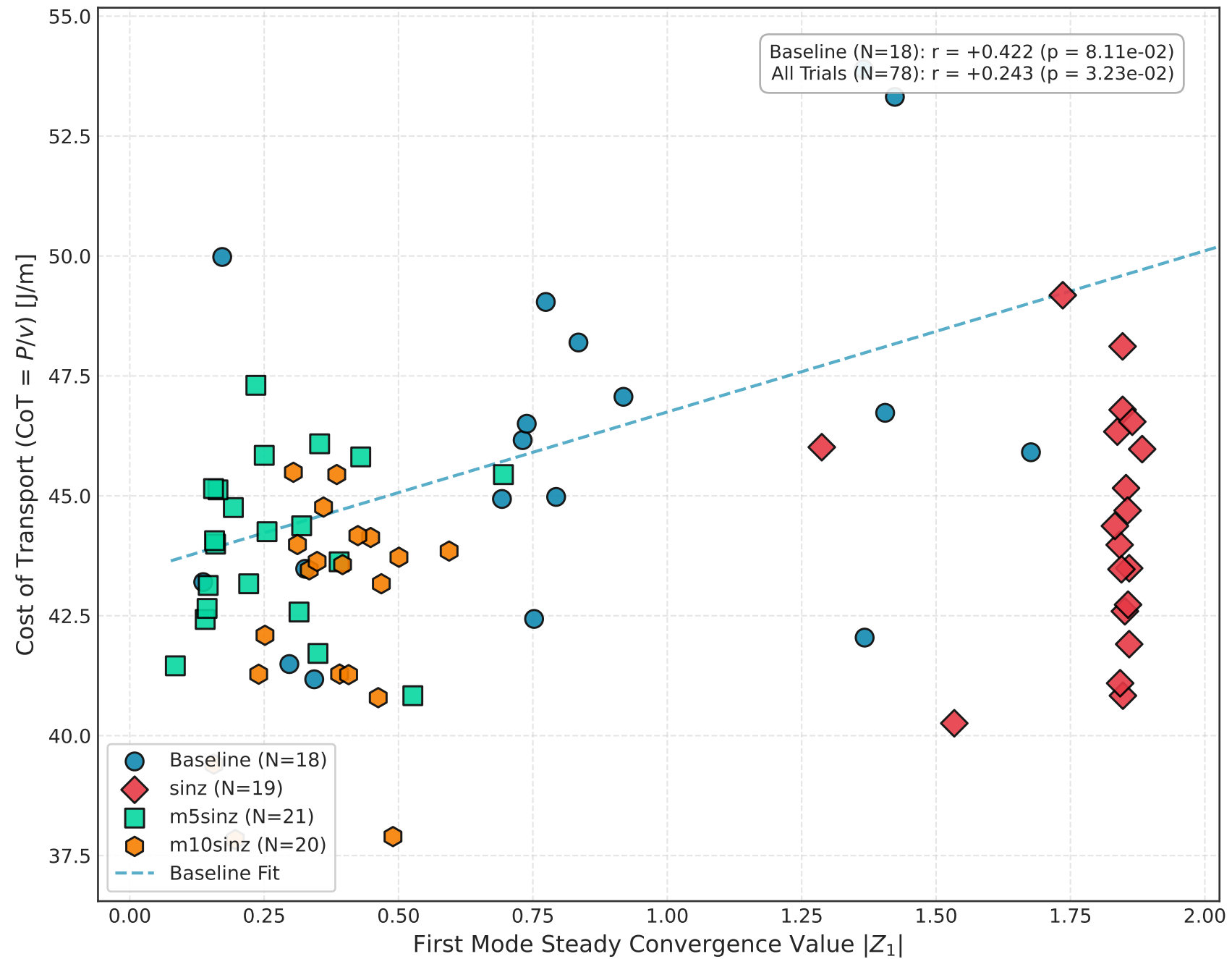
First Mode Convergence Value vs. Cost of Transport
