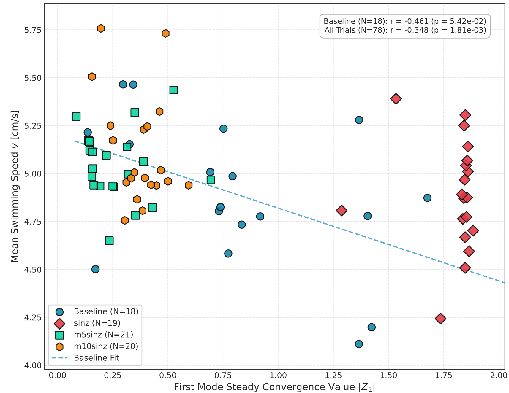
First Mode Convergence Value vs. Swimming Speed
