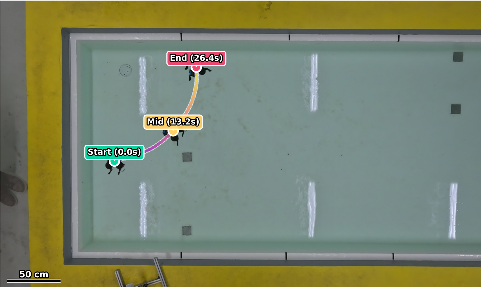
Baseline (No coupling) (GX011337) Speed: 4.87 cm/s, Dist: 1.30 m, CoT: 45.91 J/m
