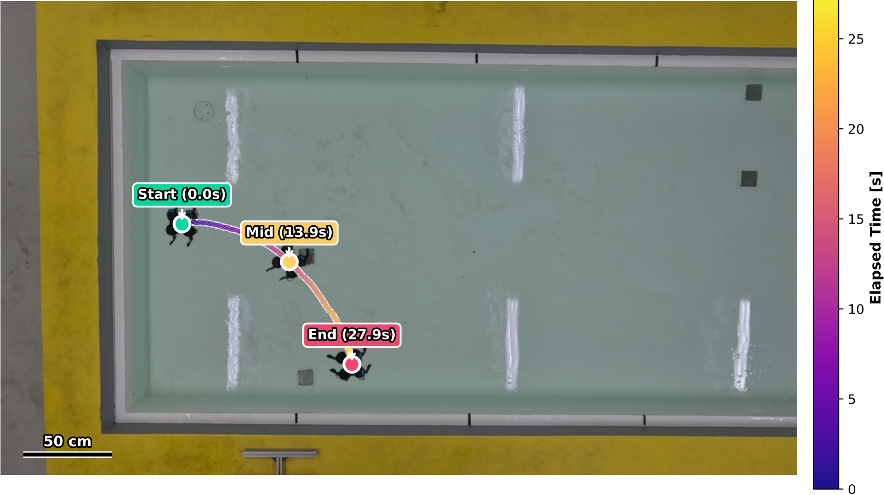
\sin(\theta) ( M = 1 ) (GX011388) Speed: 4.89 cm/s, Dist: 1.38 m, CoT: 44.37 J/m
