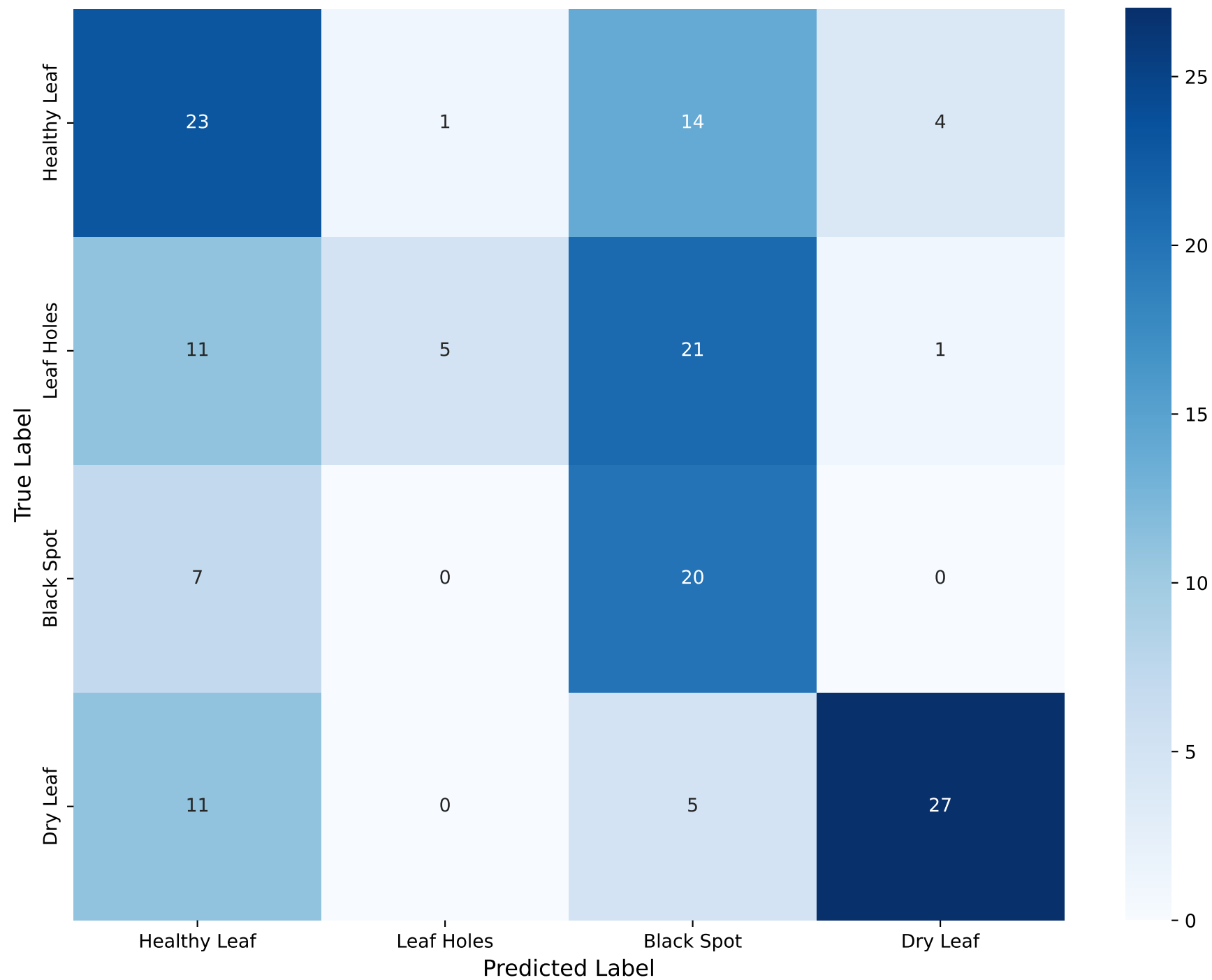
Confusion Matrix - Test Set
