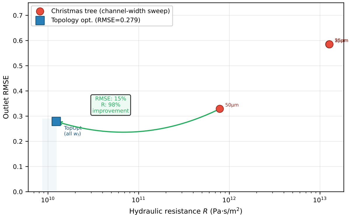
Performance comparison: topology optimisation vs. best-achievable Christmas-tree design (channel-width sweep)
