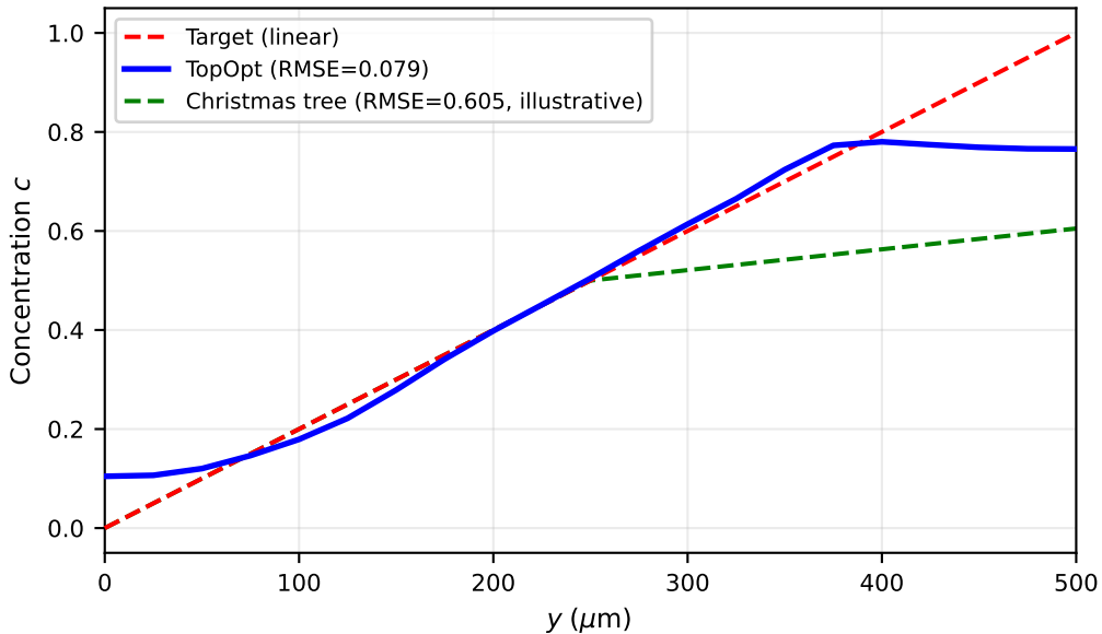
Outlet profiles: TopOpt vs Christmas-tree baseline
