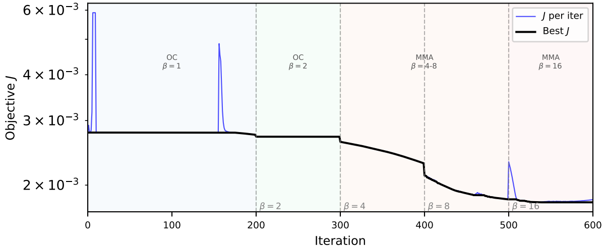
Convergence history — hybrid OC/MMA, 600 iterations
