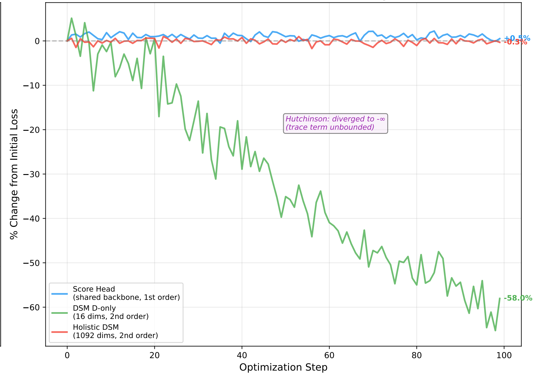
DSM Alternatives: Relative Change
