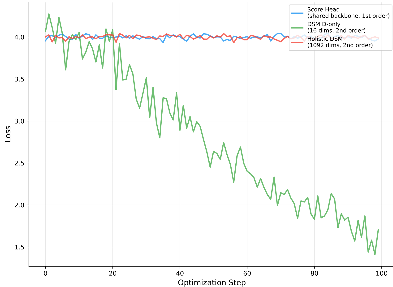
DSM Alternatives: Raw Loss (Hutchinson excluded — diverged to -\infty )
