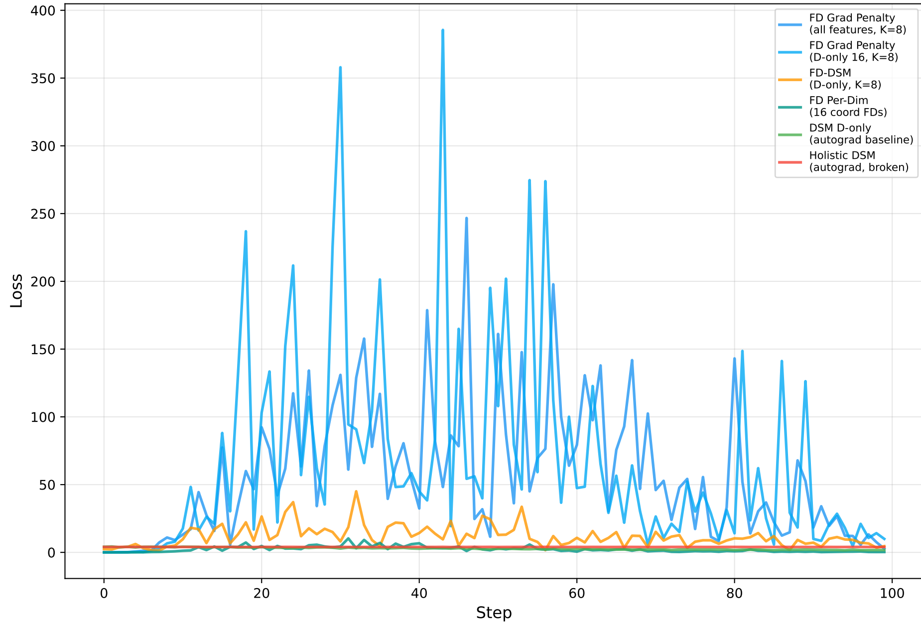
FD vs Autograd DSM: Raw Loss
