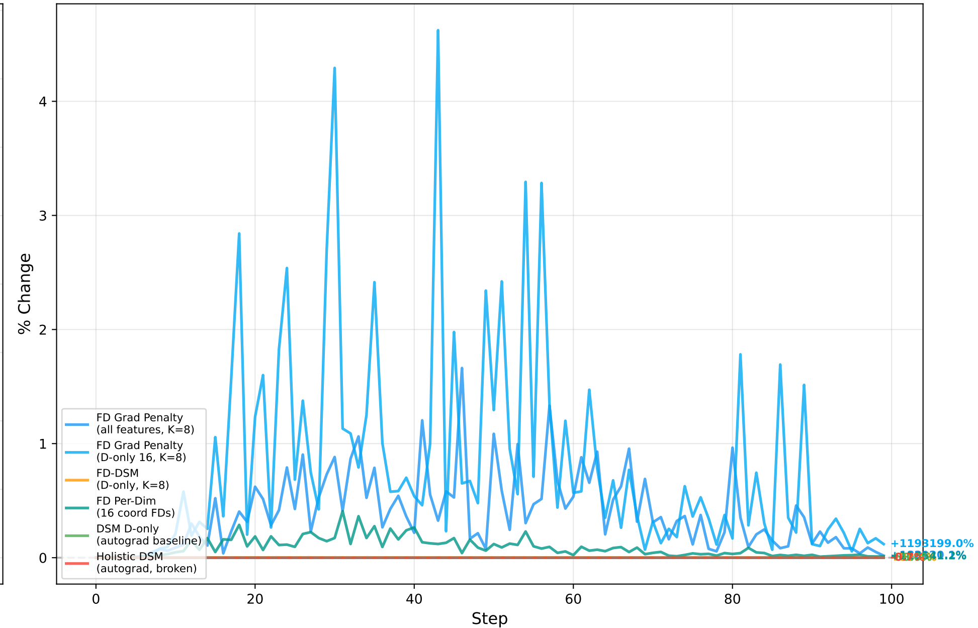
FD vs Autograd DSM: Relative Change
