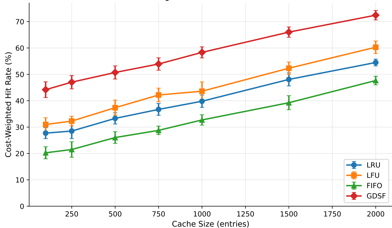
Cost-Weighted Hit Rate vs Cache Size
