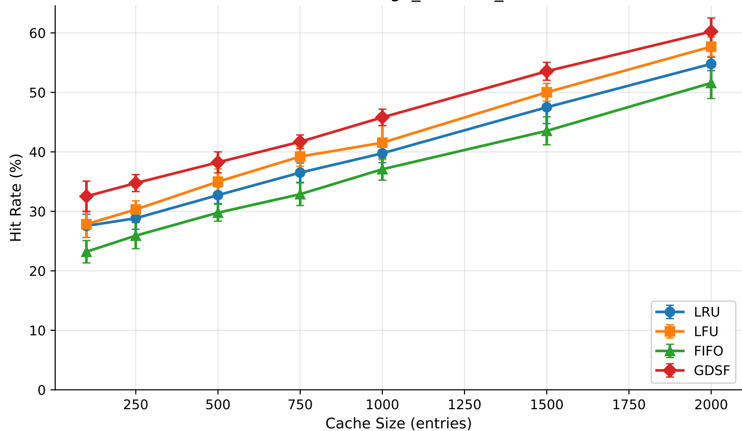
Hit Rate vs Cache Size (high_variance_cost workload)
