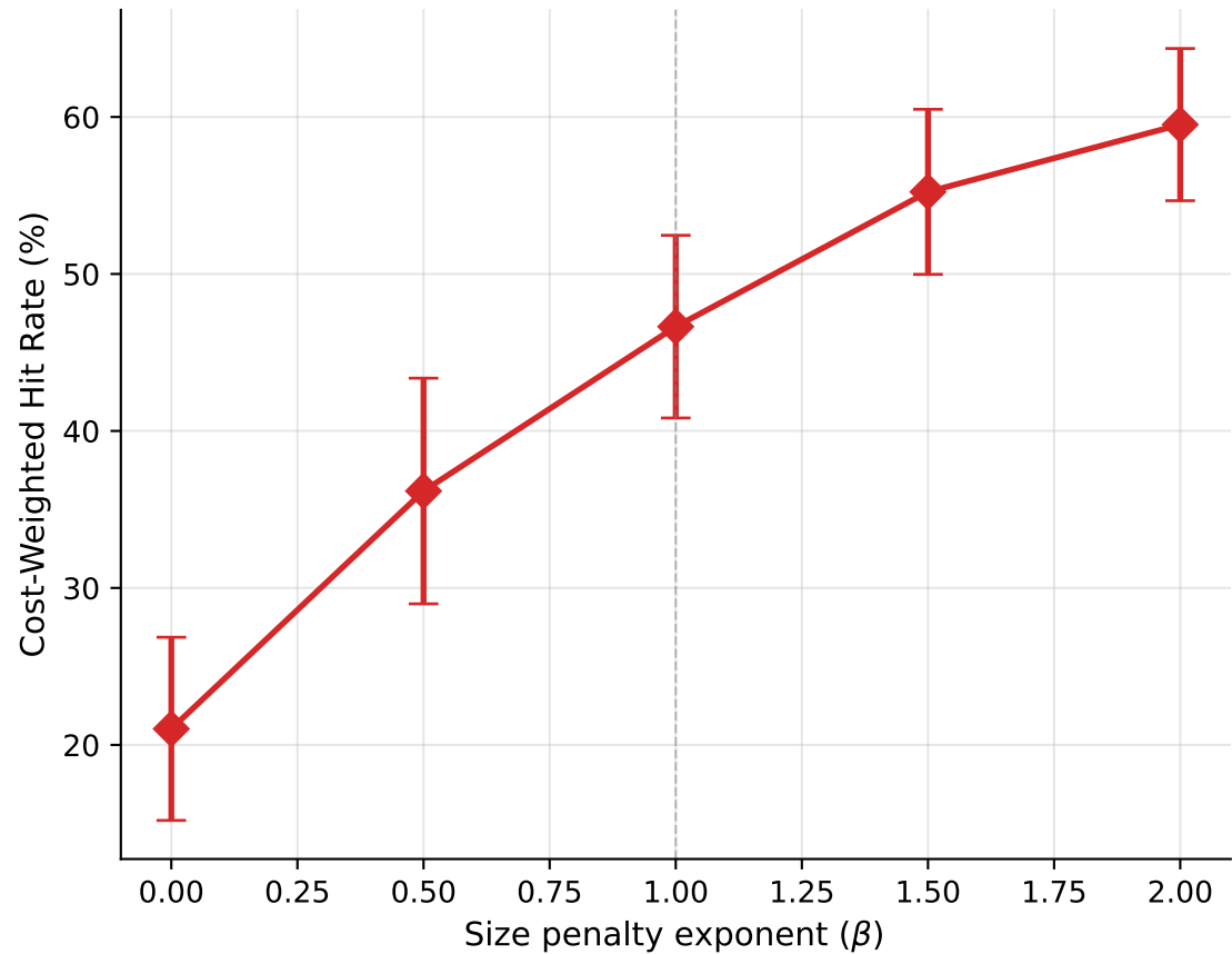
Sensitivity to \beta ( \alpha=1.0 )
