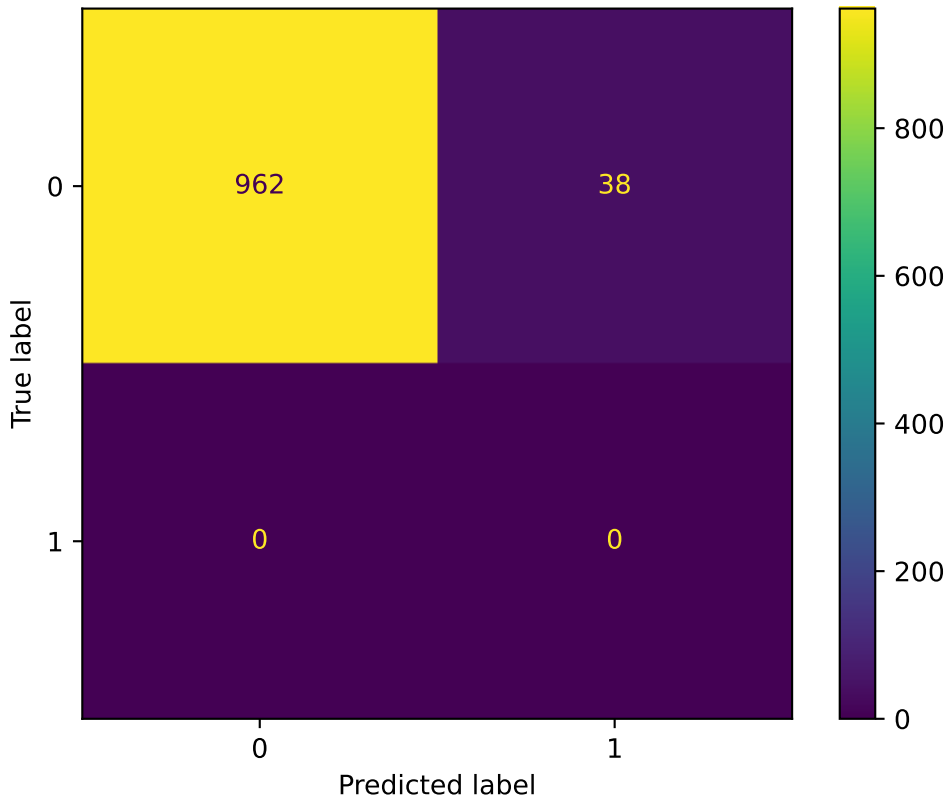
Confusion Matrix - Software Model
