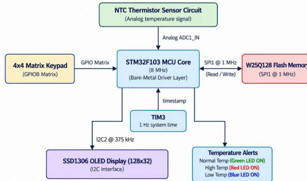
Figure 1. Functional architecture: sensor acquisition, processing, timestamping, buffering, non-volatile storage, user interface, and temperature alerts.
