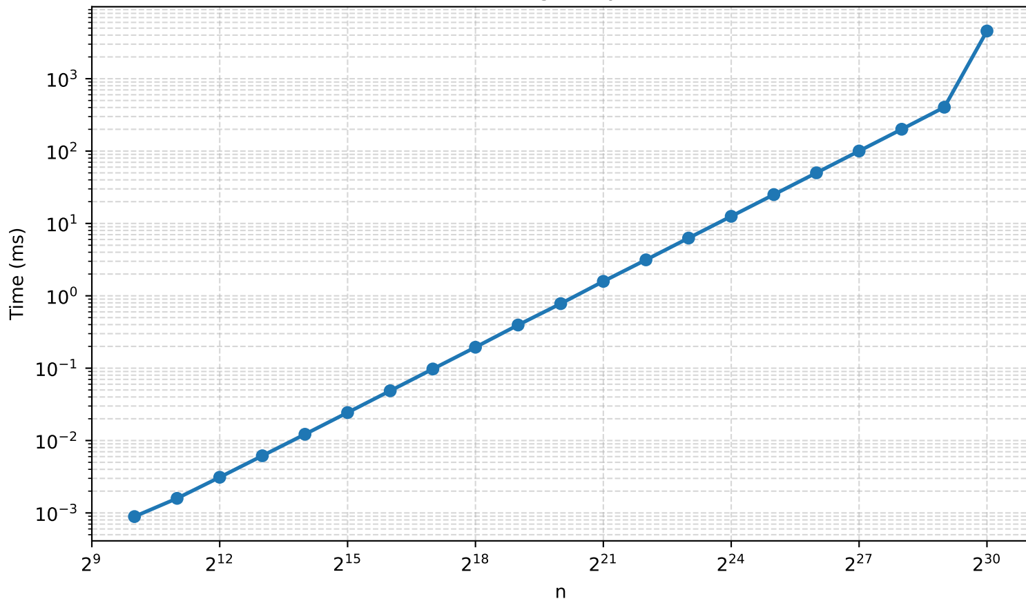
Scaling Analysis
