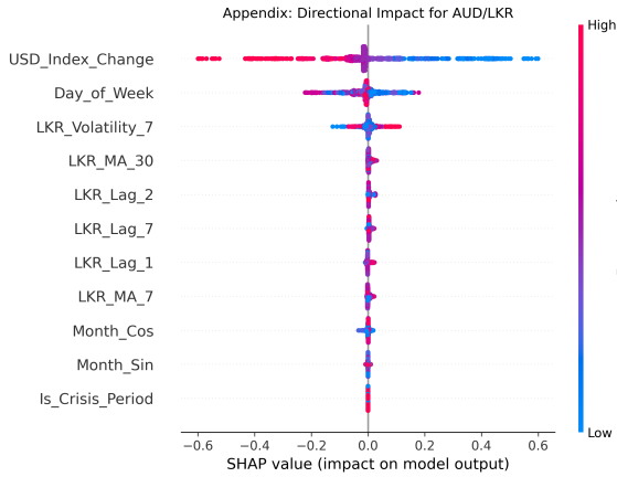
(e) AUD/LKR Impact Distribution
