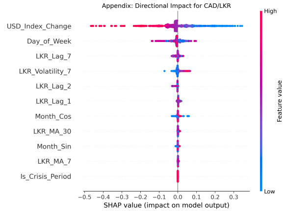
(f) CAD/LKR Impact Distribution
