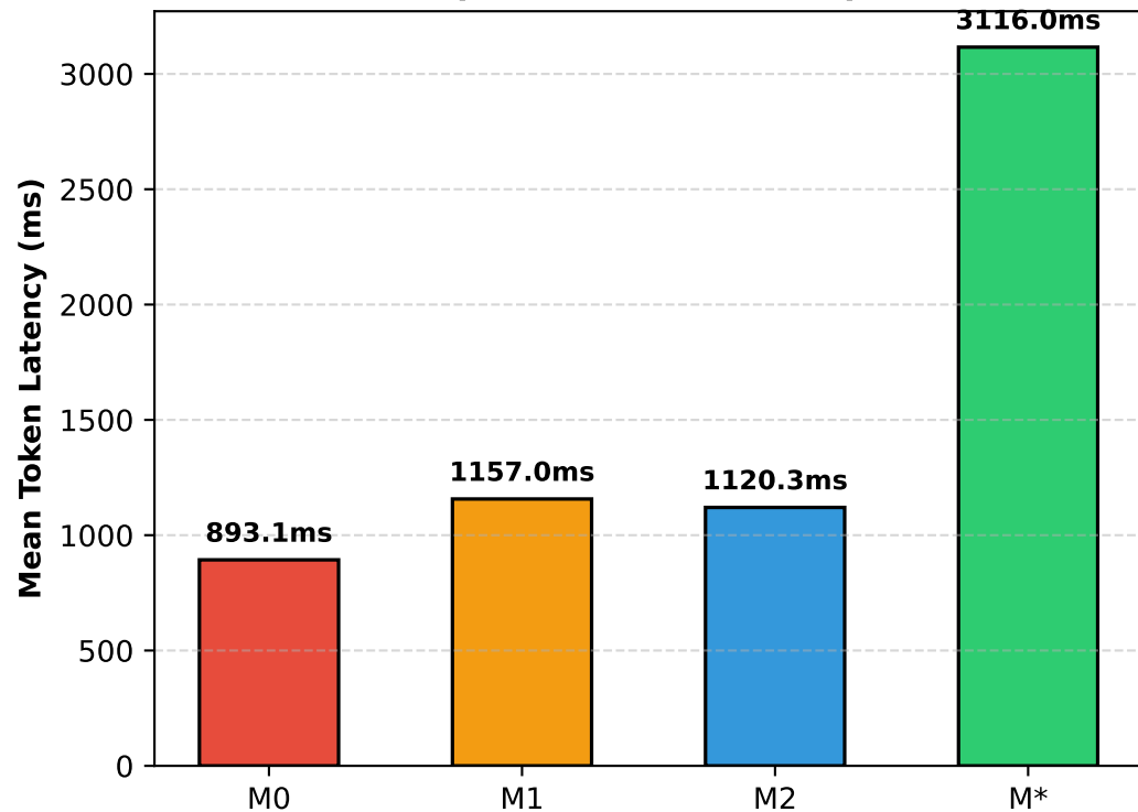
(b) Computational Overhead per Call
