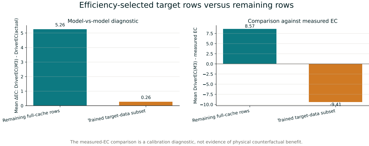
Figure C.4: Lead-1 M3 -via- M2 counterfactual subset diagnostic.
