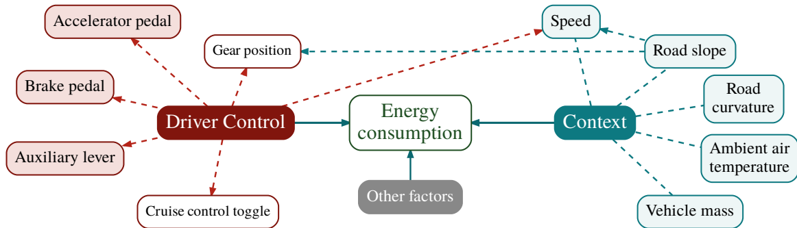
Figure 1.1: Energy consumption (EC) depends on operating-context factors and driver-control signals.
