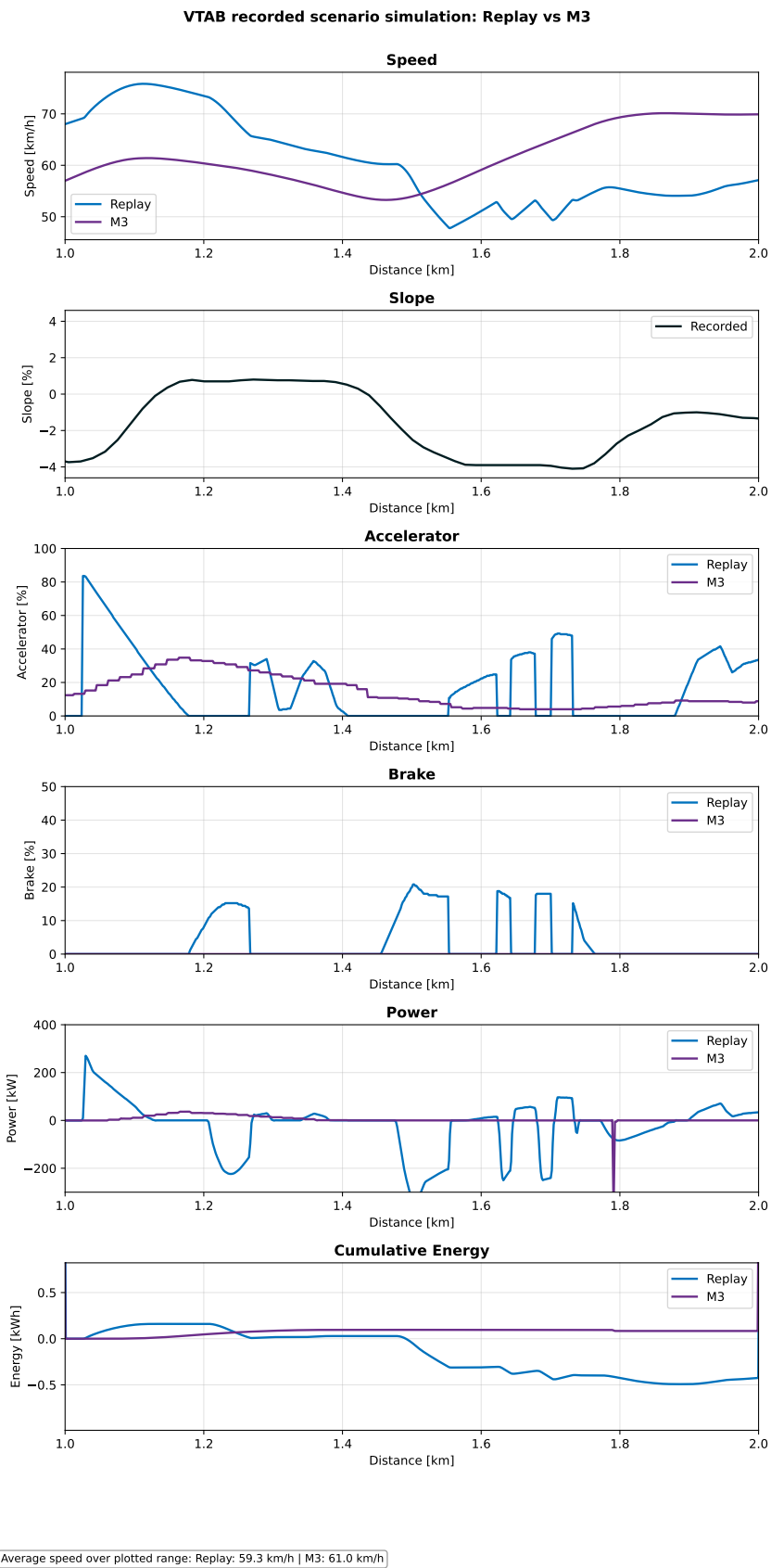
Figure C.6: Second recorded-route replay case, zoomed segment 1 (1.0–2.0 km).
