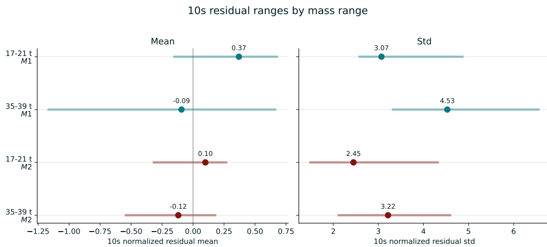
Figure A.3: Normalized residual ranges by mass range.
