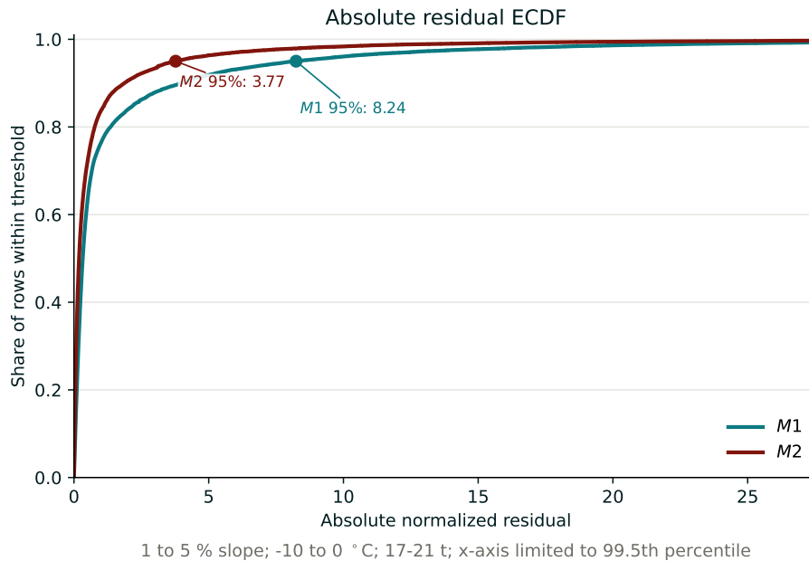
Figure A.1: Absolute normalized residual ECDF for the selected 17–21 t bucket.
