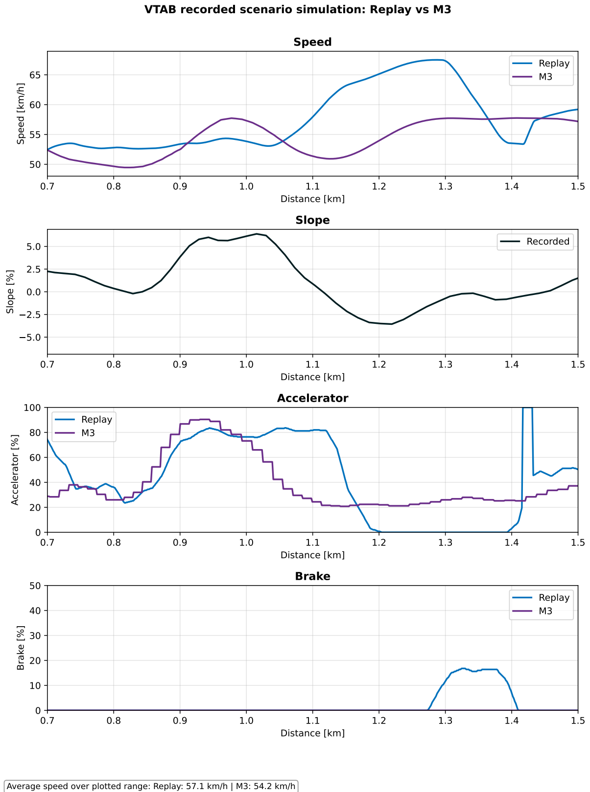
Figure 4.13: Zoomed simulation traces from 0.7 to 1.5 km.
