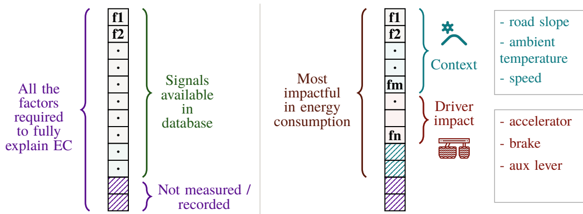
Figure 3.1: Feature-selection logic for context and driver-control modeling.
