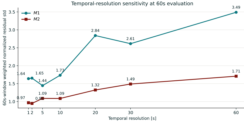
Figure B.1: Weighted 60 s-window normalized residual standard deviation for M1 and M2 under feature resolutions from 1 s to 60 s.
