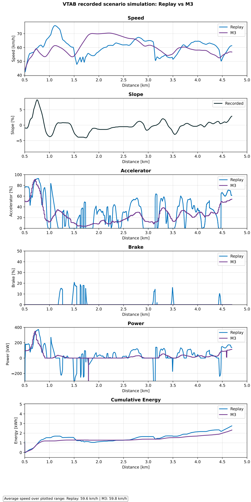
Figure C.5: Second recorded-route replay case: speed, slope, accelerator, brake, power, and cumulative energy for replay and M3 .
