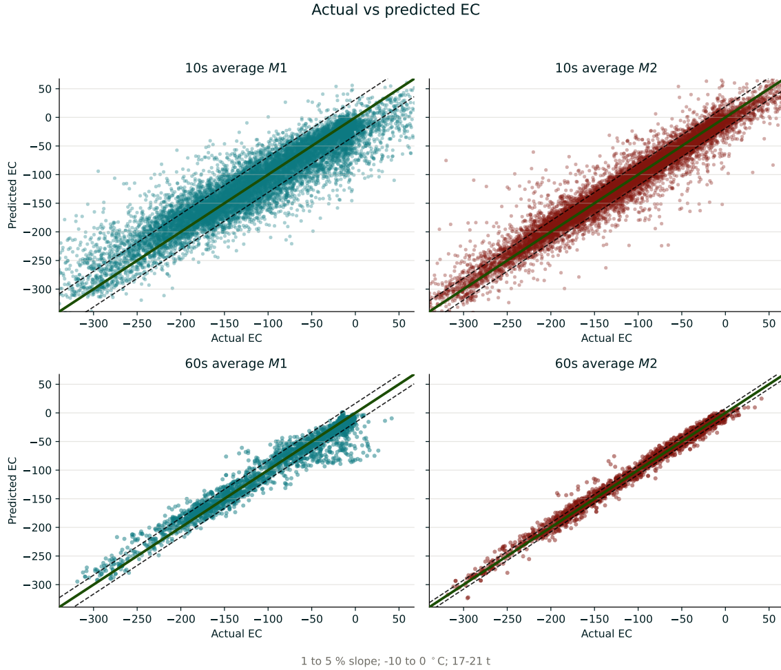
Figure 4.1: Actual and predicted energy consumption at 10 s and 60 s averaging scales.
