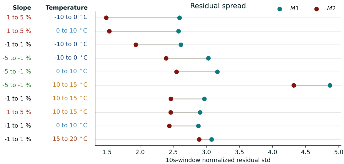
Figure 4.2: Normalized residual standard deviation for M1 and M2 across the primary 17–21 t comparable-condition buckets.
