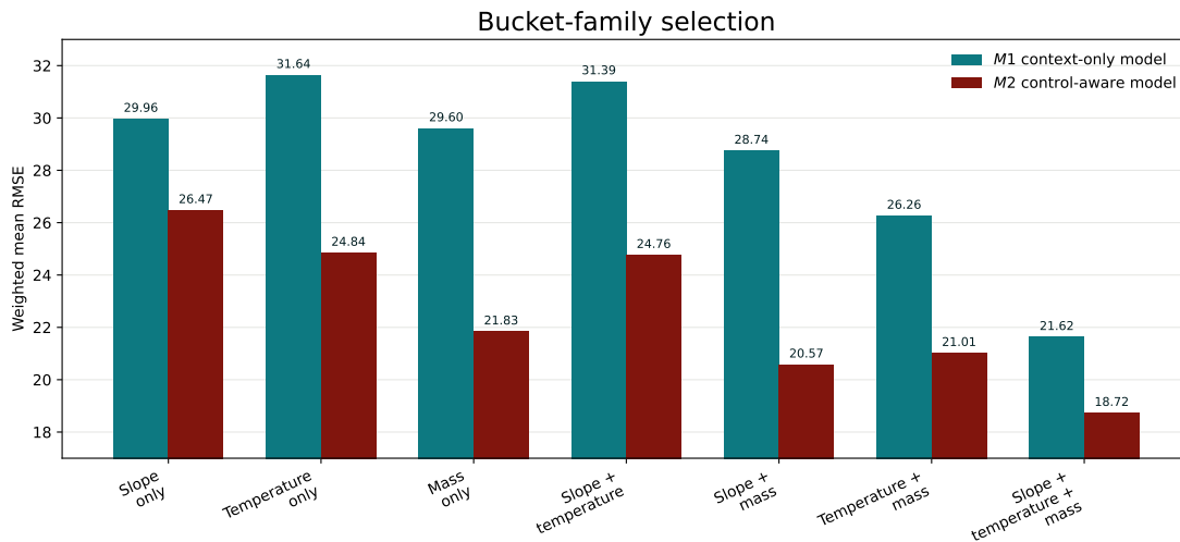
Figure 4.3: Weighted mean RMSE by bucket family.
