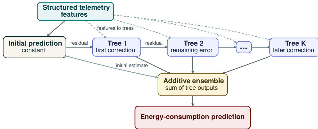
Figure 2.2: Additive boosted-tree prediction structure.
