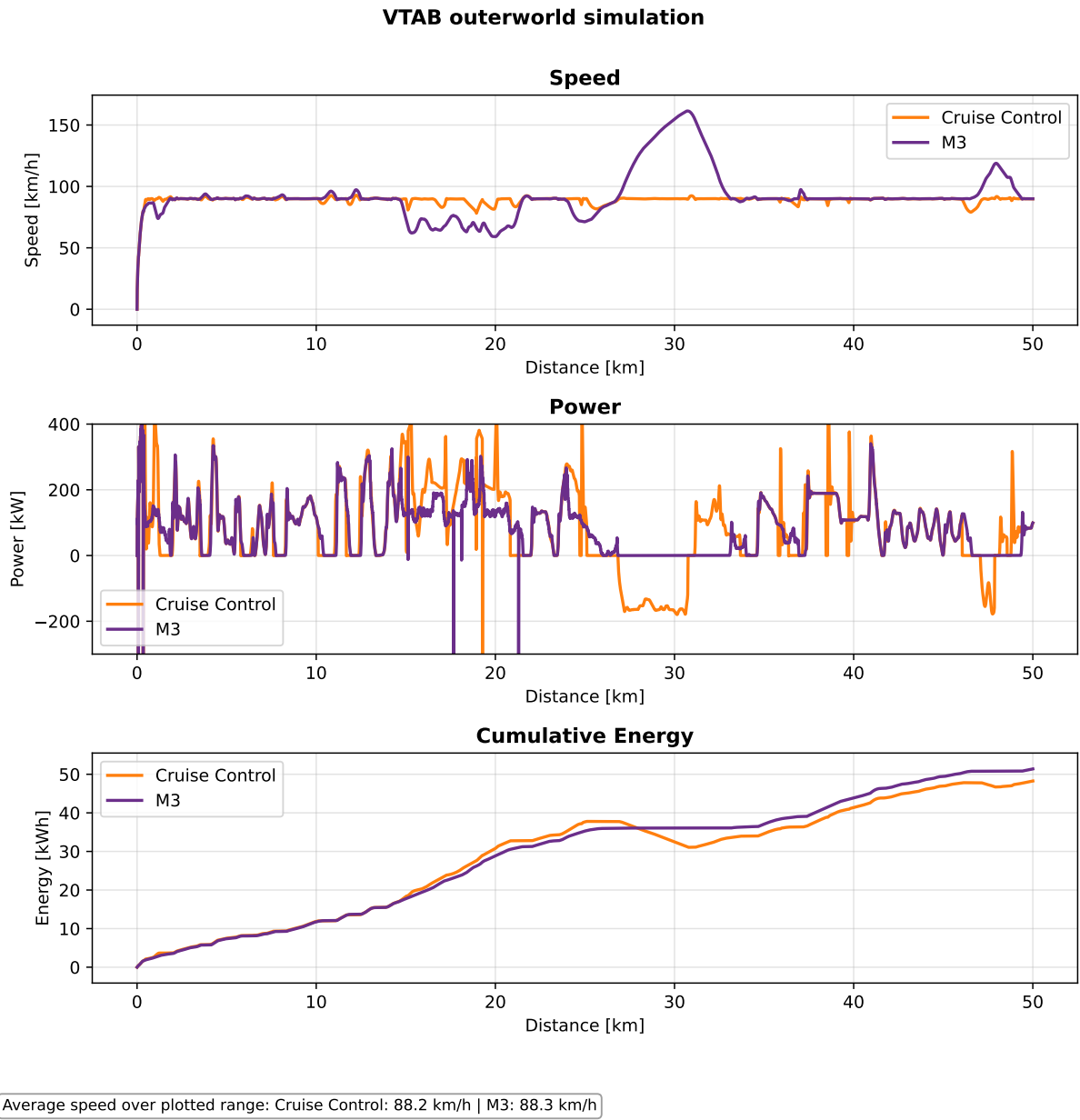
Figure 4.15: Distance-based OuterWorld simulation traces for CCAP and M3 .
