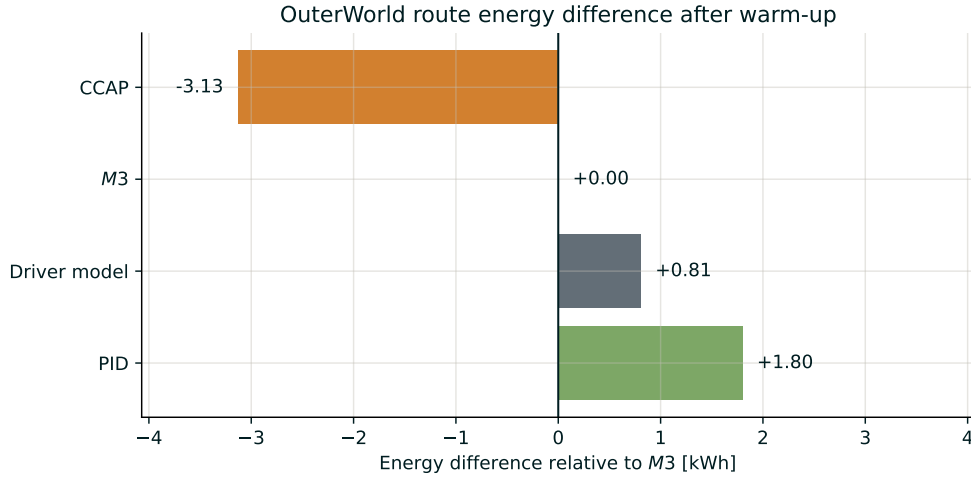
Figure 4.14: Post-warm-up cumulative-energy difference on the VTAB OuterWorld route.
