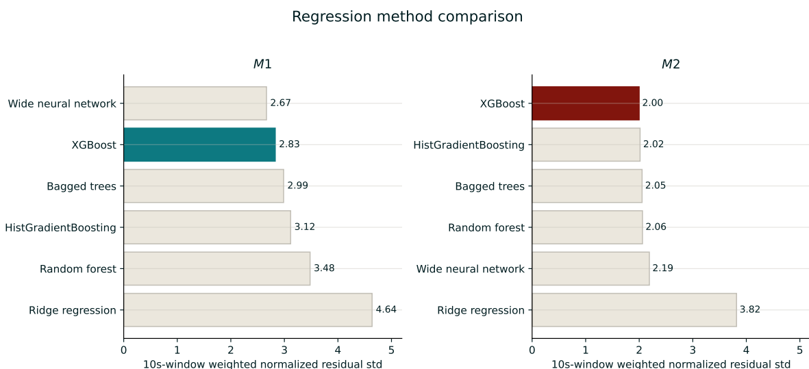
Figure 4.8: Weighted normalized residual standard deviation by supervised regression method for M1 and M2 .
