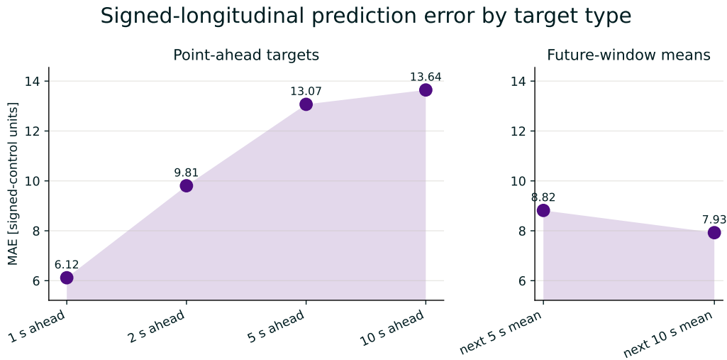
Figure C.1: Signed-longitudinal MAE by prediction horizon.
