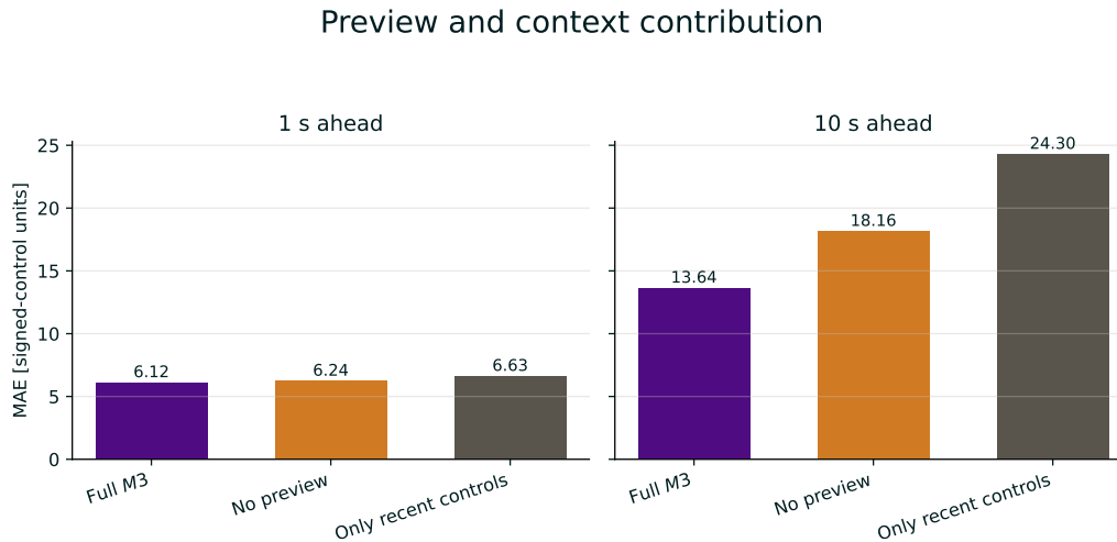
Figure 4.10: Signed-longitudinal MAE for the full M3 model and reduced feature variants at 1 s and 10 s ahead.
