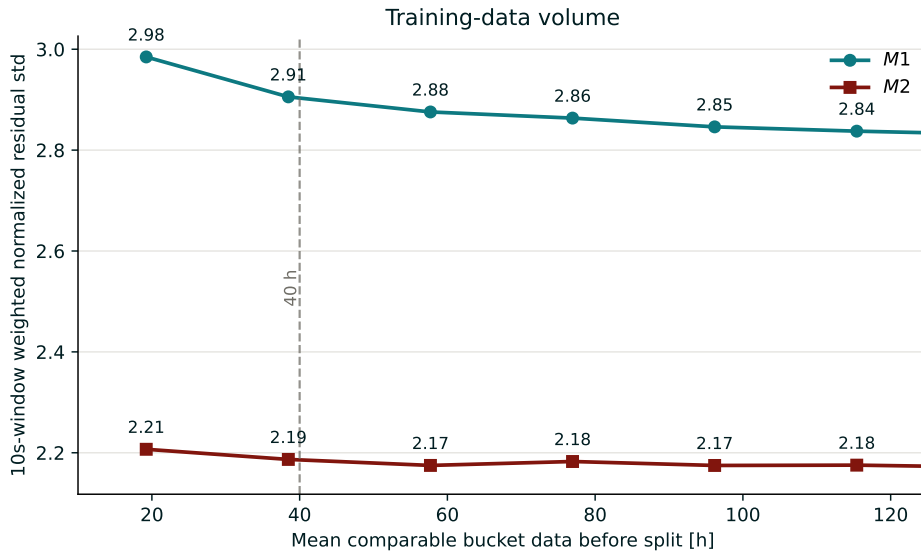
Figure 4.6: Aggregate 10 s-window normalized residual spread across comparable bucket-data volume.
