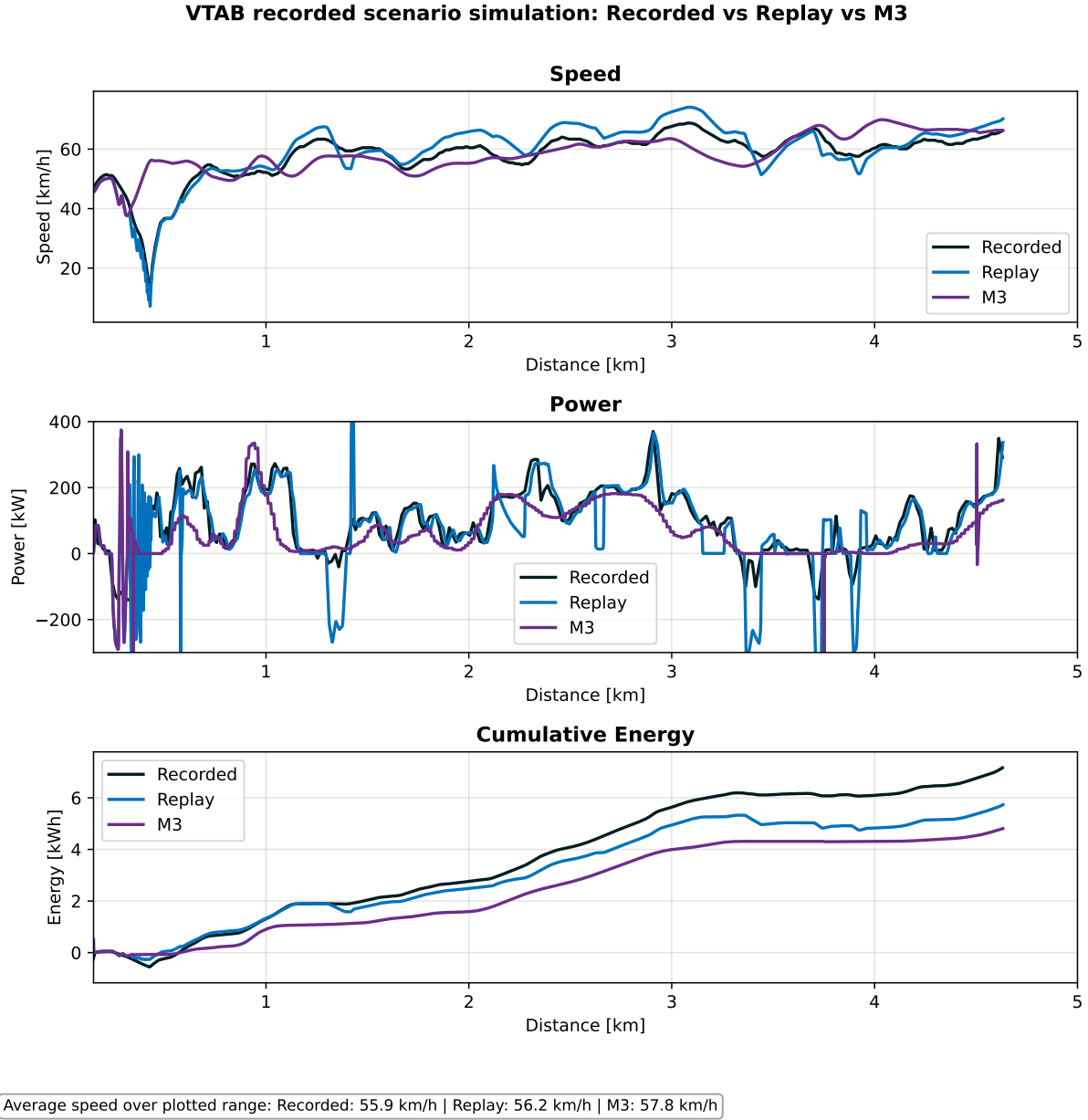
Figure 4.12: Distance-based simulation traces for recorded data, replay baseline, and M3 .
