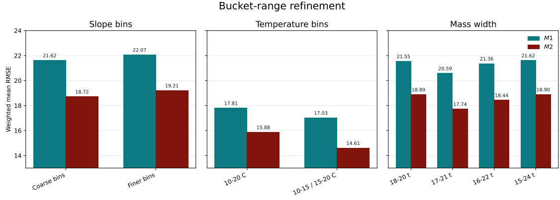
Figure 4.4: Weighted mean RMSE for bucket-range refinement tests.
