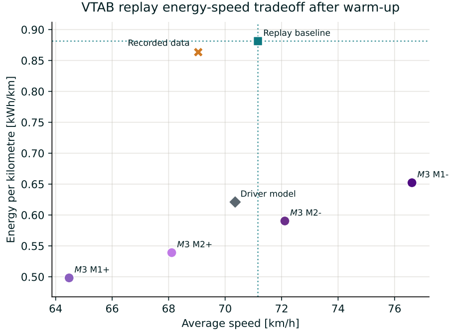
Figure 4.11: Post-warm-up energy intensity and average speed for replay window 2.
