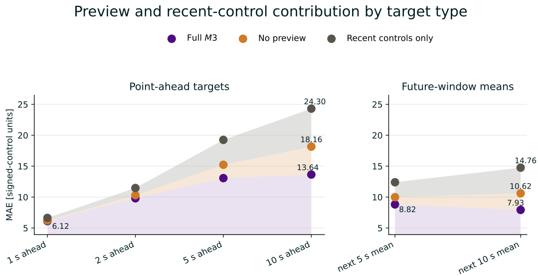
Figure C.2: Signed-longitudinal MAE by prediction horizon for the full M3 model, the no-preview variant, and the recent-controls-only variant.
