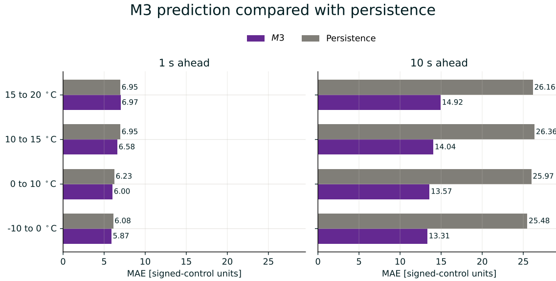
Figure 4.9: Signed-longitudinal MAE for M3 and a persistence baseline at 1 s and 10 s prediction horizons.
