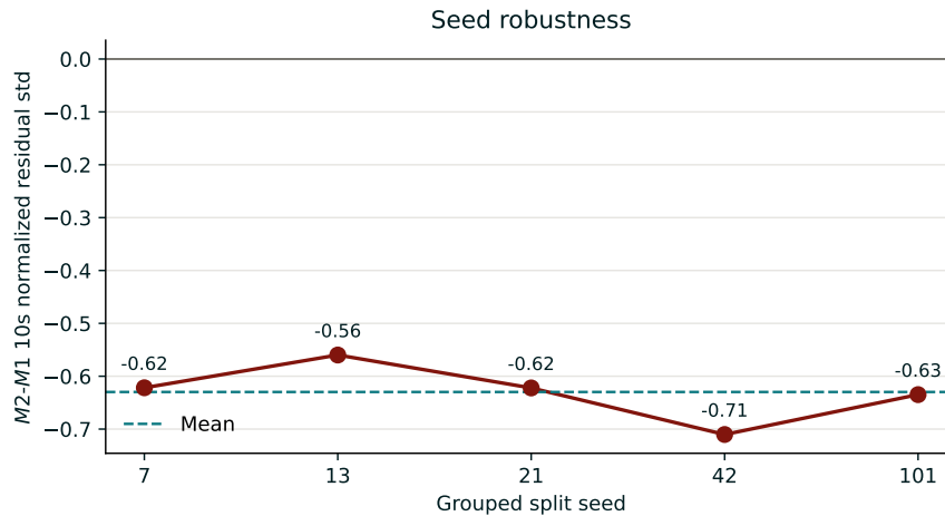
Figure A.2: Grouped-split seed robustness for normalized residual spread.
