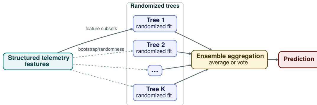
Figure 2.1: Conceptual schematic of a random-forest ensemble, based on Breiman [28].
