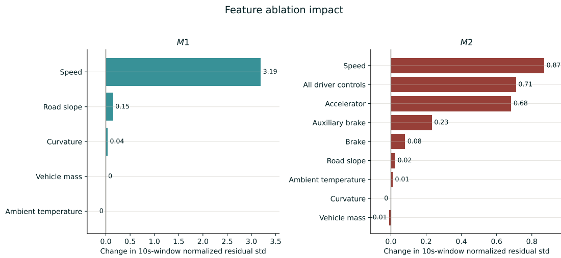
Figure 4.7: Change in weighted 10 s-window normalized residual standard deviation after feature-group ablation.
