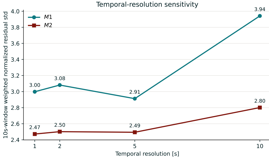
Figure 4.5: Weighted normalized residual standard deviation for M1 and M2 under reduced feature resolutions.
