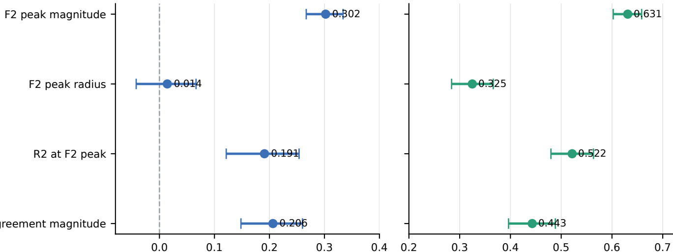
A. Variance recovery ( R^2 )
