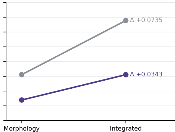
Balanced accuracy
