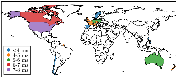
Figure 23: Global GS ↔ PoP latencies from Starlink RIPE Atlas probes.
