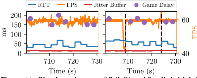
Figure 11: Cloud gaming over 5G (left) and Starlink (right). Vertical dashed lines show Starlink reconfiguration intervals.
