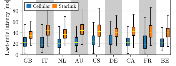
Figure 12: Last-mile latencies for different countries. “Starlink” denotes satellite bent-pipe over RIPE Atlas while “Cellular” wireless access from Speedchecker [10].
