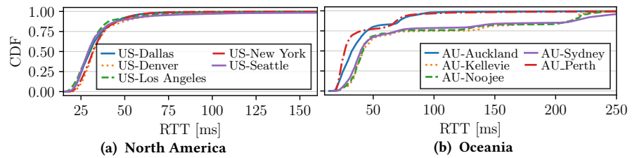
Figure 22: The distribution of the minimum RTT (minRTT) during M-Lab measurements from selected cities in North America (a) and Oceania (b).
