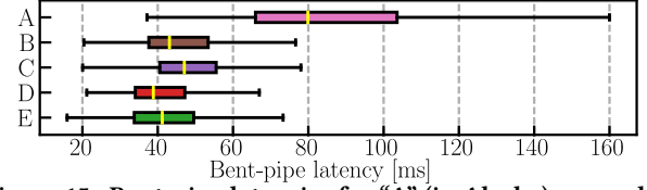
Figure 15: Bent-pipe latencies for “A” (in Alaska) covered by the 70^\circ and 97.6^\circ while the rest (Sweden “B”, Canada “C”, UK “D”, and Germany “E”) are also covered by 53^\circ .
