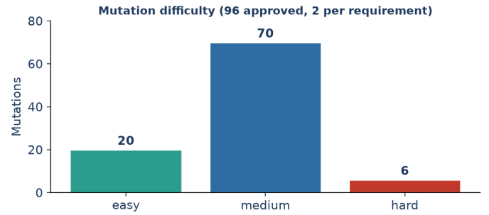
Fig. 3. Mutation difficulty distribution across the 96 approved mutations.
