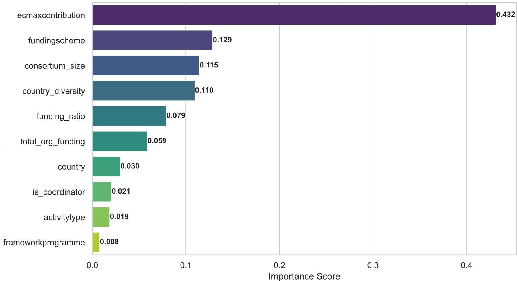
Feature Importance for Predicting Project Duration
