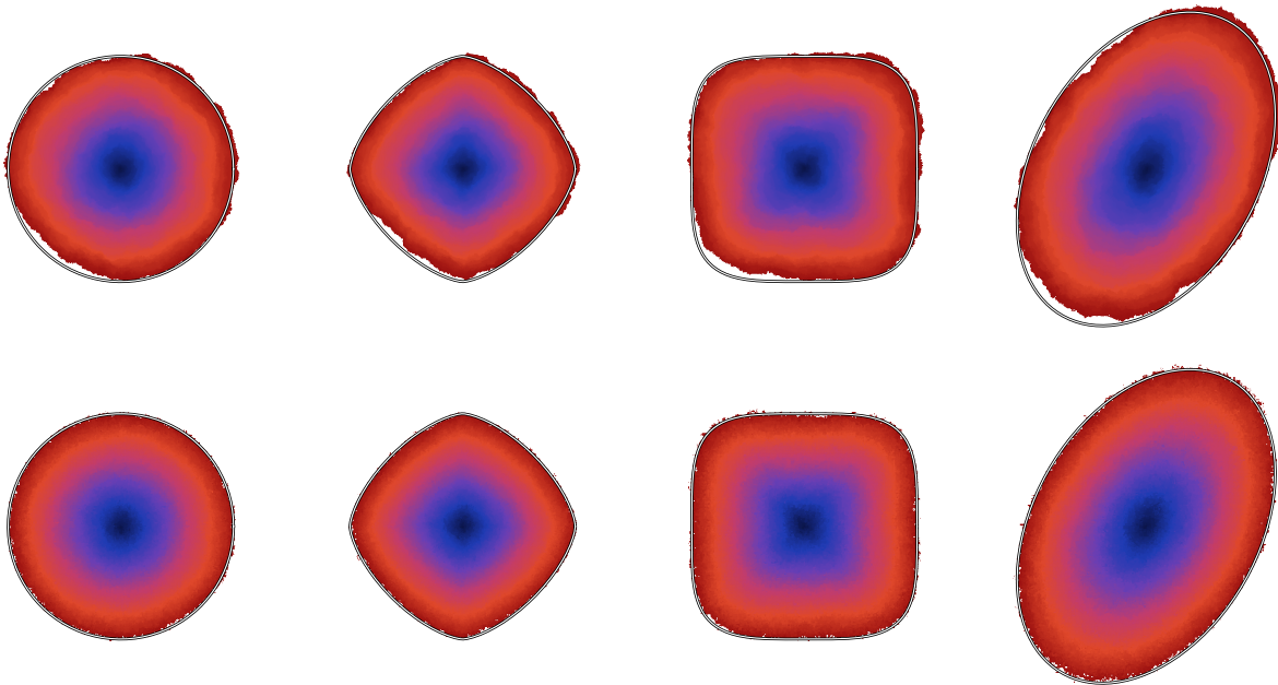
FIGURE 2. Ranges r_n^{-1}A_n for the Euclidean, \ell^{3/2} , \ell^4 and elliptical norms (left to right), at n = 10^9 . Top: d = 2 , \kappa = 0.4 ; bottom: x_3 = 0 sections for d = 3 , \kappa = 0.25 . The unit balls are outlined and the blue-to-red colors show (t_x/n)^{1/(d+1)} , with t_x the first-departure time.
