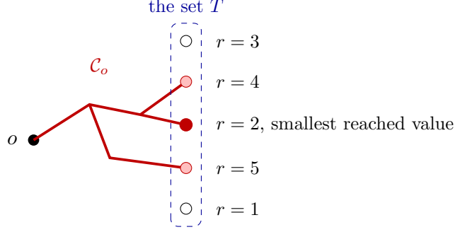
Figure 8: Selection by the ordering r . The cluster of o reaches three vertices of T , drawn filled, and misses two, drawn open. Among the reached vertices, the one with smallest r -value has r = 2 . The vertex with r = 1 is not reached.
