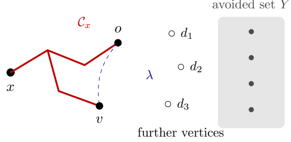
Figure 7: The data of Theorem 4.9. The cluster of x is forbidden to reach the shaded set Y , drawn as the shaded region on the right. The vertices o and v are compared: the value of the conditional covariance at the first is bounded below by the value at the second, discounted by the number \lambda . The vertices d_1, \dots, d_\ell of Section 4.3 are the open circles, and the constant attached to d_j is computed with d_1, \dots, d_{j-1} already avoided.
